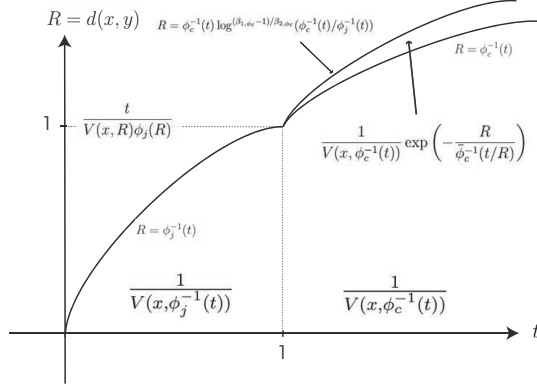
Figure 1: Dominant term in the heat kernel estimates \text{HK}(\phi_j, \phi_c) for p(t, x, y) for the case in Remark 1.17.
