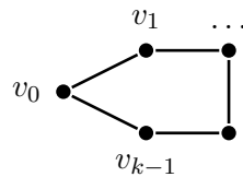
cycle with k = 5 vertices and edges
