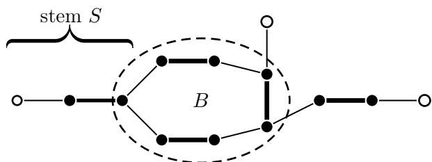
matching M with M -blossom B
