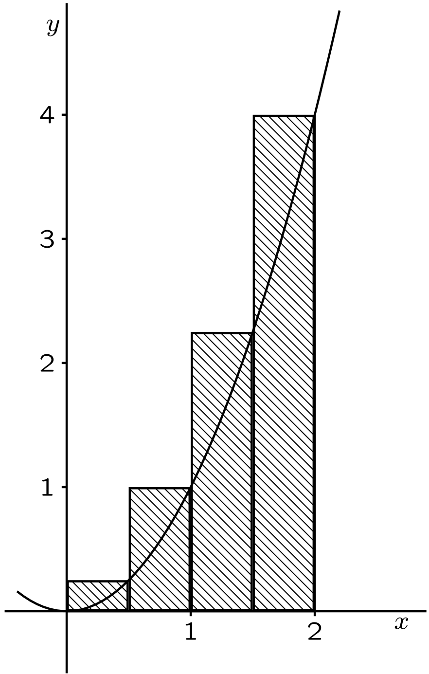
n = 4 , right endpoints
