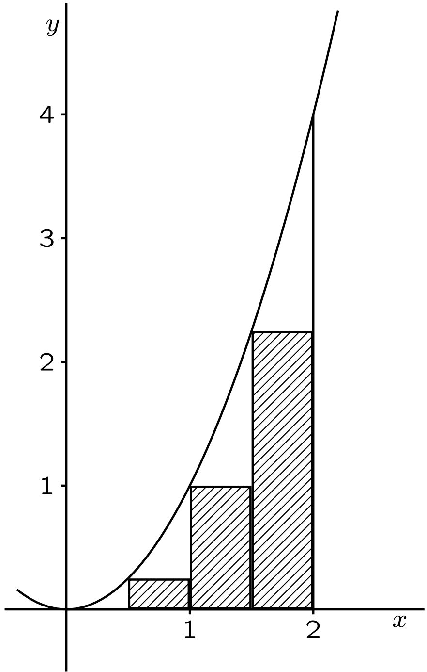
n = 4 , left endpoints
