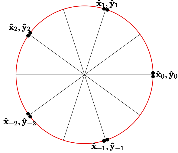
Figure 1: The Gale diagram of Q_3
