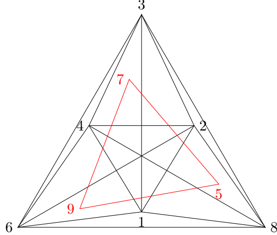
Figure 3: The affine Gale diagram of \mathcal{P}_{42}^0
