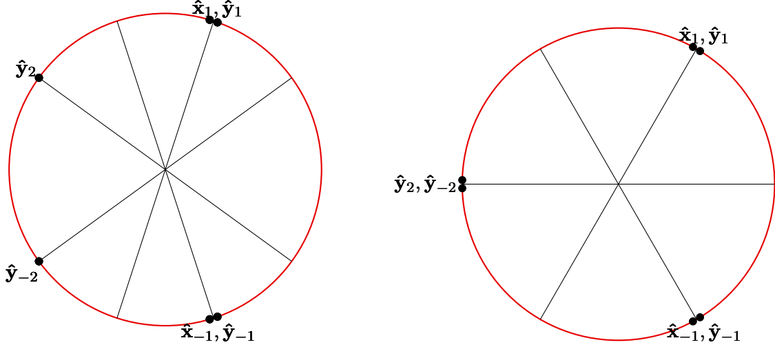
Figure 2: The Gale diagram C_3 \setminus (\hat{e}_1 \cup \hat{e}_2) and an equivalent Gale diagram
