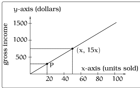
(a) Gross income graph.
