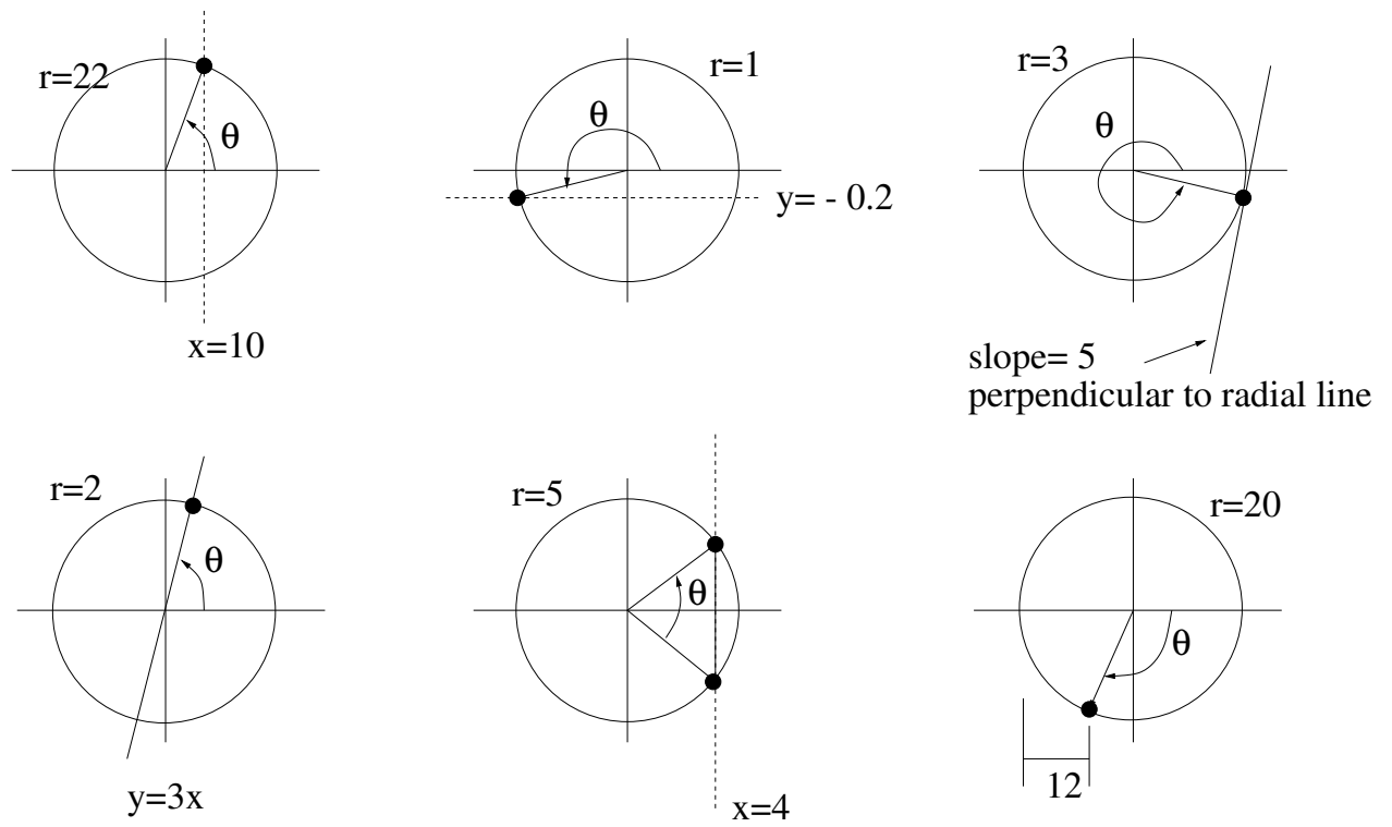
Figure 18.14: Circles for Exercise 18.14.
