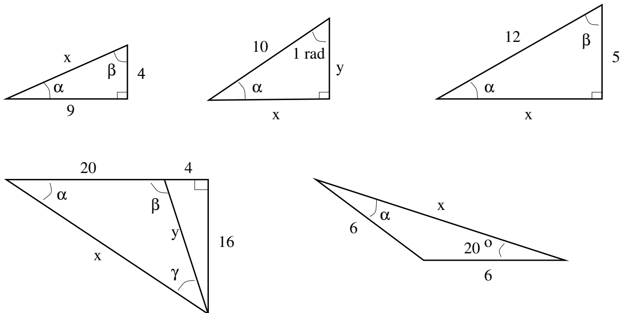
Figure 18.15: Triangles for Exercise 18.15.
