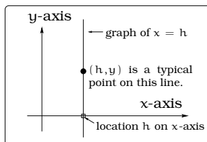
(a) Vertical line.
