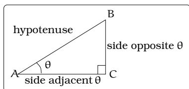
Figure 15.3: Labeling the sides of a right triangle.
