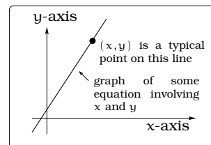
(c) Sloped line.
