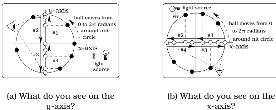
Figure 16.3: Analyzing the values of the sine and cosine functions.
