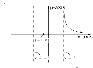
Figure 12.4: The graph of g(x) on the right of x = 3 .
