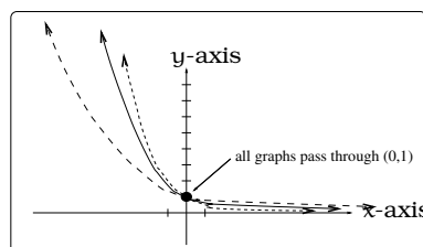
(b) Graph of y = b^x , 0 < b < 1 .
