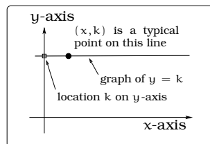
(b) Horizontal line.
