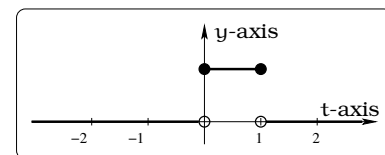
Figure 10.7: A basic step function u(t) .
