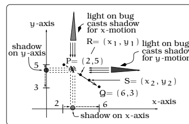
(b) How to view motion in the coordinates.
