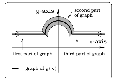
Figure 6.12: Multipart function g(x) .
