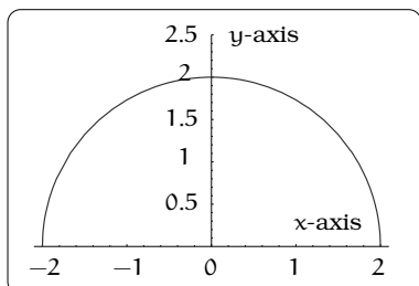
Figure 9.7: Graph of y = \sqrt{4 - x^2} .
