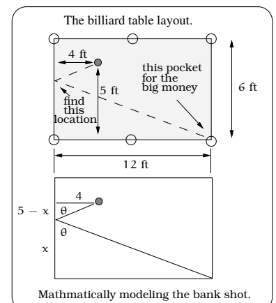
Figure 15.2: A pocket billiard banking problem.
