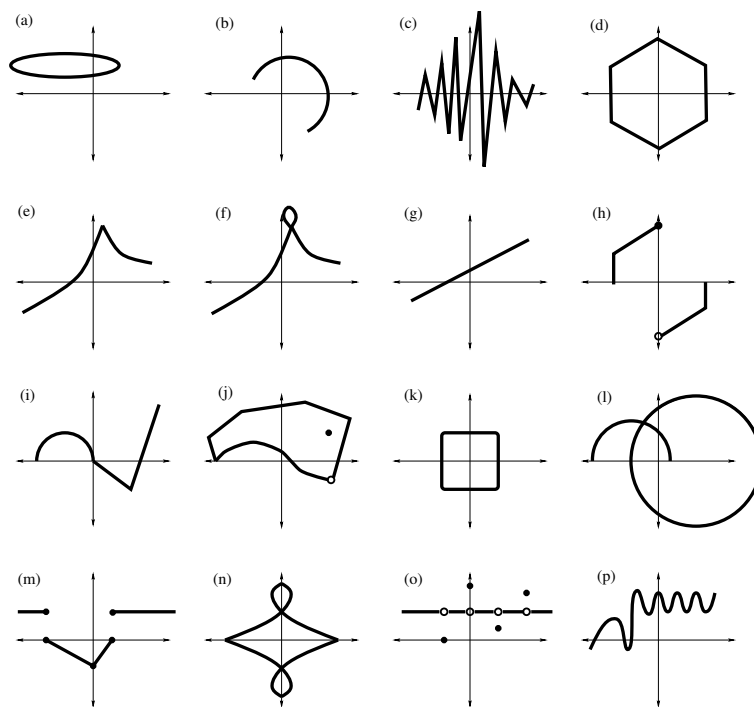
Figure 5.14: Curves to consider for Problem 5.12
