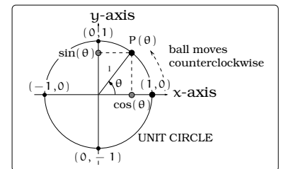
Figure 16.1: Visualizing the range of \sin(\theta) and \cos(\theta) .
