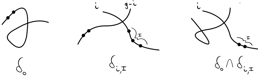
Figure 5.21: Examples of stable curves in the boundary.
