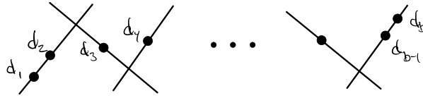
Figure 5.27: The degenerate curve (D, d_i) \in \overline{M}_{0,b}
