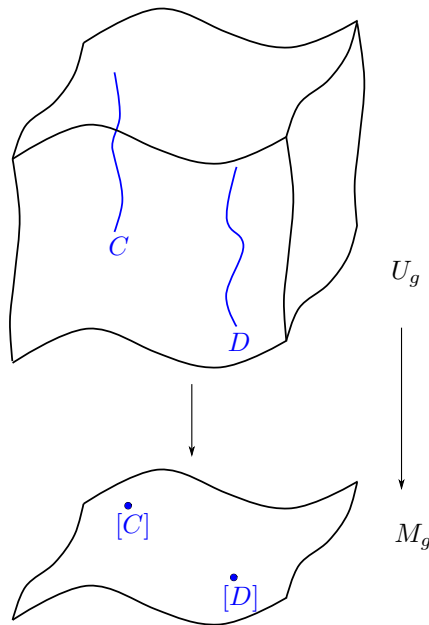
Figure 0.11: Visualization of a (non-existent) universal family over M_g .
