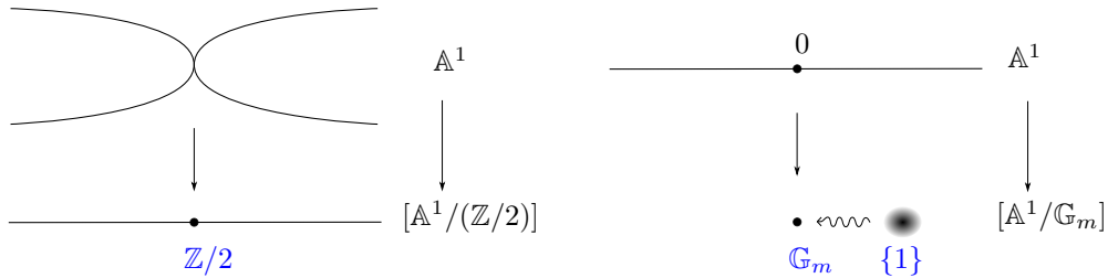
Figure 0.13: Pictures of the scaling actions of \mathbb{Z}/2 = \{\pm 1\} and \mathbb{G}_m on \mathbb{A}^1 over \mathbb{C} with the automorphism groups listed in blue. Note that [\mathbb{A}^1/\mathbb{G}_m] has two isomorphism classes of objects—0 and 1—corresponding to the two orbits—0 and \mathbb{A}^1 \setminus 0 —such that 0 \in \{1\} if the set \mathbb{A}^1/\mathbb{G}_m is endowed with the quotient topology.
