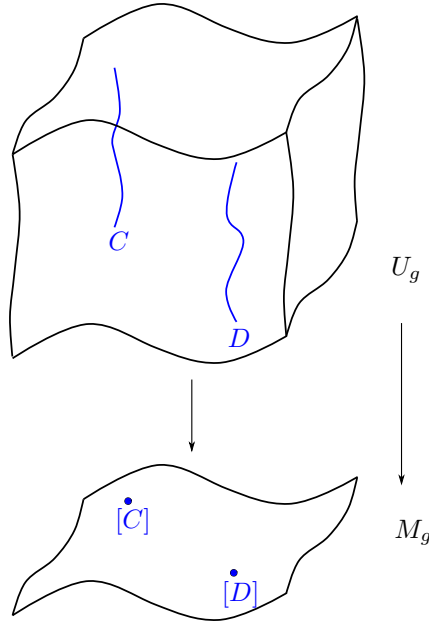
Figure 0.3.25: Visualization of a (non-existent) universal family over M_g .
