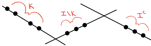
Figure 5.7.24: A curve in \delta_{0,I} \cap \delta_{0,K} as long as K \subsetneq I .
