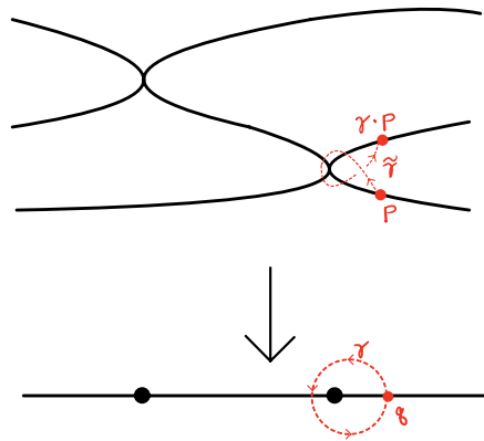
Figure 5.7.8: Monodromy action
