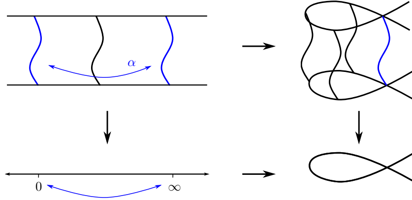
Figure 0.3.35: Family of curves over the nodal cubic obtaining by gluing the fibers over 0 and \infty of the trivial family over \mathbb{P}^1 via \alpha . (It would be more illustrative to draw a Möbius band as the family of curves over the nodal cubic.)
