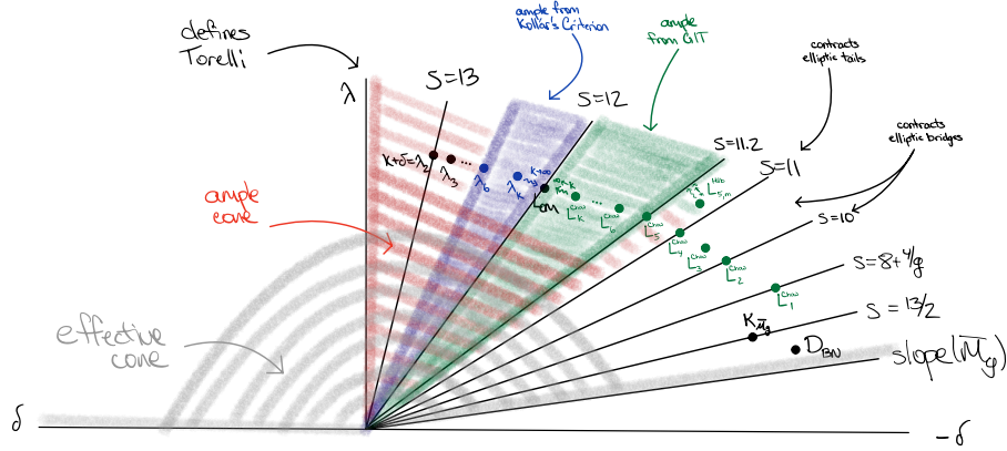
Figure 5.10.12: Ample and effective cone of \overline{M}_g in the \lambda - \delta -plane.
