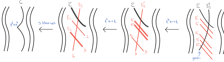
Figure 5.5.14: The numbers indicate the multiplicity of a component; if no number is given, the multiplicity is 1. The thickened components indicate the ramification locus under the normalized base change.
