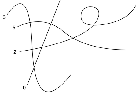
Figure 5.2.13: An example of a nodal curve of genus 14.
