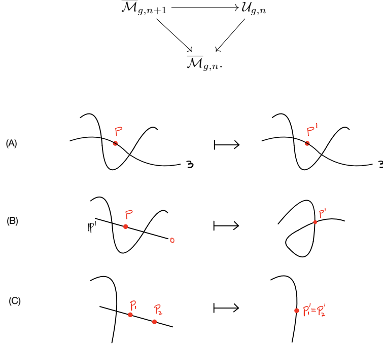
Figure 5.6.11: Examples of the map \overline{\mathcal{M}}_{g,n} \rightarrow \mathcal{U}_{g,n} .
