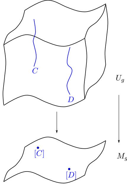
Figure 0.3.27: Visualization of a (non-existent) universal family over M_g .
