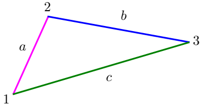
Figure 0.2.5: To keep track of the labeling, we color the edges.
