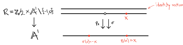
Figure 3.4.4: The quotient X = \mathbb{A}^1/R looks like \mathbb{A}_{\mathbb{R}}^1 except that the origin has residue field \mathbb{C} .
