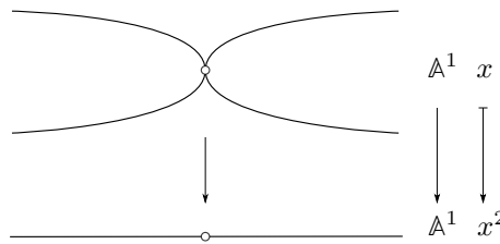
Figure 0.5.1: Picture of an étale double cover of \mathbb{A}^1 \setminus 0 .
