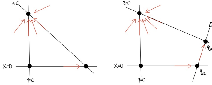
Figure 6.7.18: Białynicki-Birula stratifications for \mathbb{P}^2 (left) and \text{Bl}_p \mathbb{P}^2 (right).
