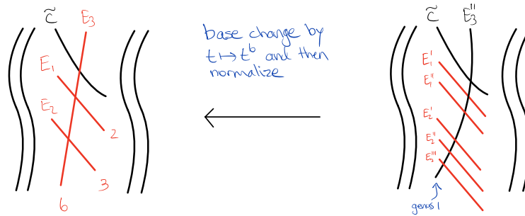
Figure 5.5.6: (Step 4) Continuing from Figure 5.5.5, we base change \mathcal{C} \rightarrow \Delta = \text{Spec} \mathbb{k}[t]_{(t)} by \Delta' = \text{Spec} \mathbb{k}[t]_{(t)} \rightarrow \text{Spec} \mathbb{k}[t]_{(t)} = \Delta , given by t \mapsto t^6 , and then normalize. The central fiber is now reduced and nodal. Each preimage of E_1 and E_2 are smooth rational curves, while the preimage E_3'' of E_3 is a genus 1 curve. To understand this description, it is convenient to break the base change into the composition of the normalized base change by t \mapsto t^2 and the normalized base change by t \mapsto t^3 , which we describe in Example 5.5.13.
