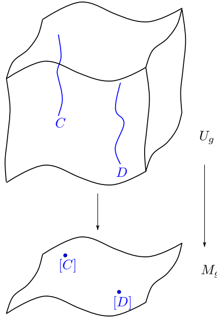
Figure 0.3.25: Visualization of a (non-existent) universal family over M_g .
