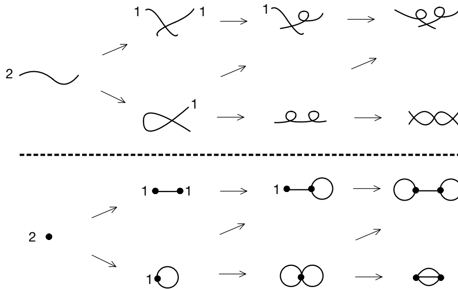
Figure 5.3.9: There are seven genus 2 vertex-weighted graphs with no marked points. Curves are displayed on the top while their dual graphs are displayed below. The arrows indicate specialization. The dimension of the substacks of \overline{\mathcal{M}}_2 parameterizing curves with a given dual graph are 3, 2, 1, and 0 in the columns going from left to right.
