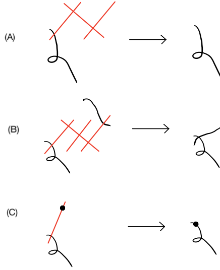
Figure 5.6.4: Stable contractions
