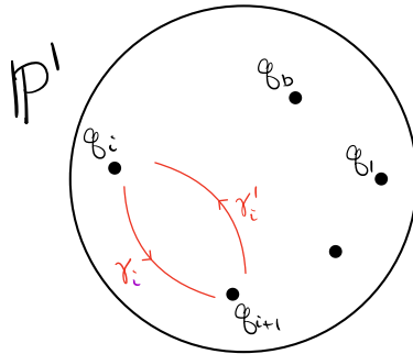
Figure 5.7.20: Paths in \mathbb{P}^1
