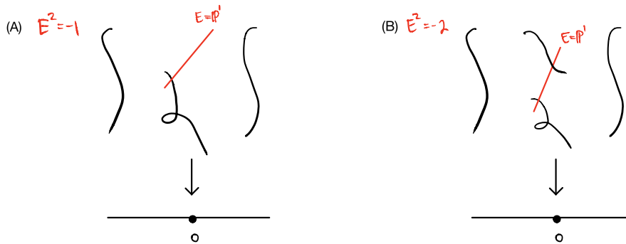
Figure 5.3.14: In (A) (resp., (B)), the exceptional component E meets the rest of the curve at one point (resp., two points) and E^2 = -1 (resp., E^2 = -2 ).
