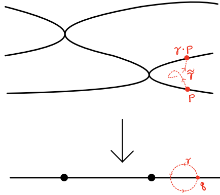
Figure 5.7.8: Monodromy action
