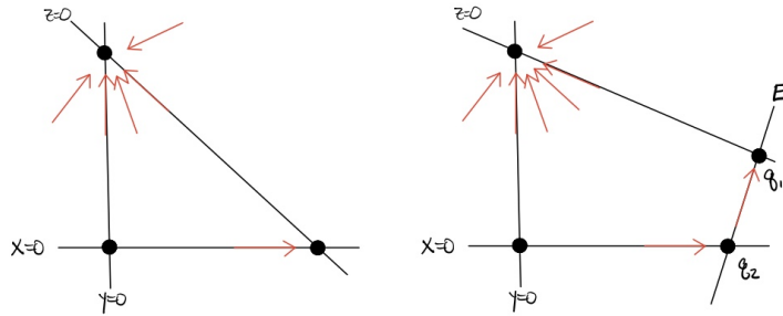
Figure 6.2: Bialynicki-Birula stratifications for \mathbb{P}^2 (left) and \text{Bl}_p \mathbb{P}^2 (right).
