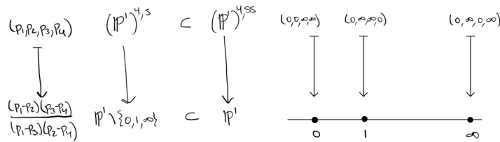
Figure 7.1: 4 unordered points up to projective equivalence
