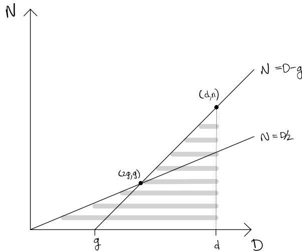
Figure 5.30: The slope of the line to (d, n) is greater than the slope to any point in the shaded areas.
