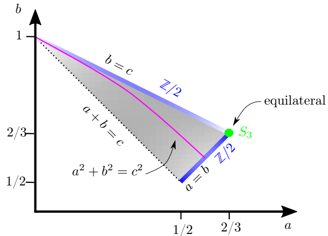
Figure 0.15: Picture of the moduli groupoid \mathcal{M}^{\text{unl}} with non-trivial automorphism groups labeled.
