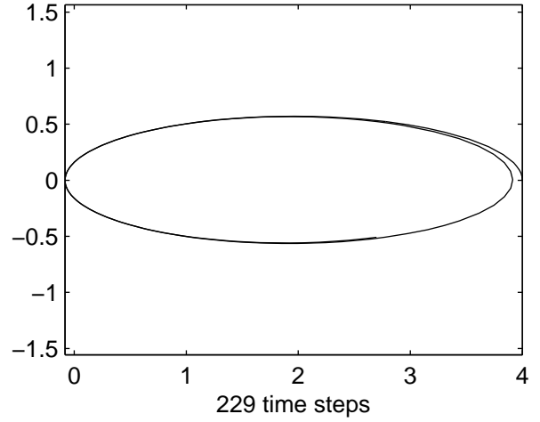
ode45 FAILS: w(0)=.01
