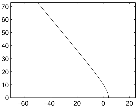
ode45: w(0)=.8
