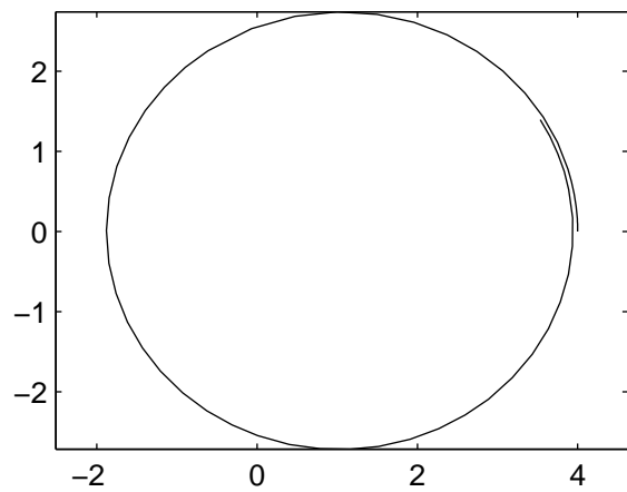
ode45: w(0)=.4
