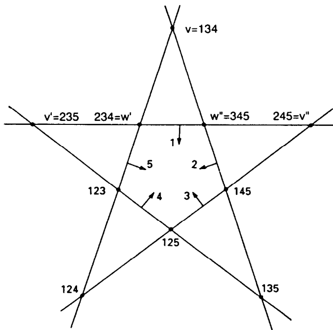
Fig. 5. An affine arrangement in \mathbb{R}^2 for which \mathcal{U}(\mathcal{M}, g) is not a lattice.
