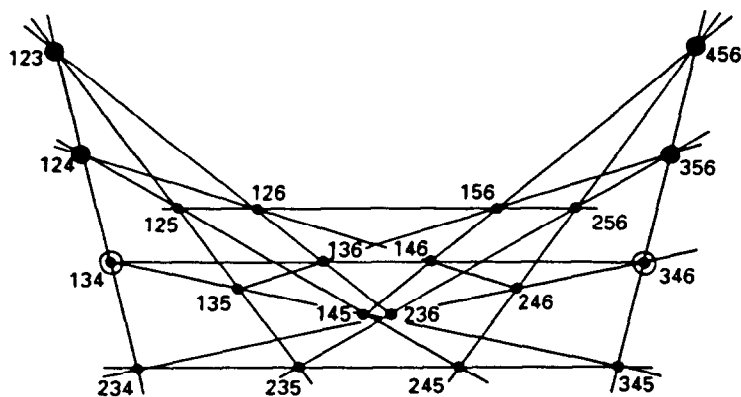
Fig. 4. The vertices and lines of B(6, 2) . The vertices marked by a black dot are in S . The vertices with a white circle are K_1 and K_6 .
