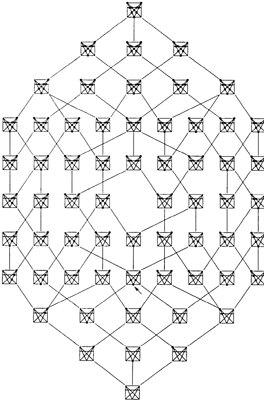
Fig. 3. The higher Bruhat order B(5, 2) .
