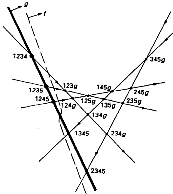
Fig. 2. The cyclic arrangement X_c^{6,2} , with g := n + 1 = 6 . The consistent set U = \{1234, 1235, 1245\} induces the extension of H_f , directions of the lines of X_c^{6,2} and thus a partial order on \binom{[5]}{3} .
