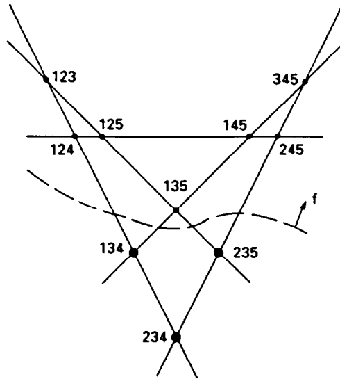
Fig. 1. The cyclic arrangement X_c^{3,2} with a pseudoline extension f and the corresponding vertex set.
