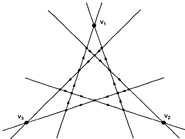
Fig. 6. An affine arrangement in \mathbb{R}^2 for which \mathcal{U}(\mathcal{M}, g) is not bounded.
