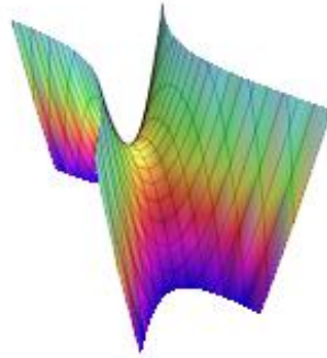
Hyperbolic paraboloid
