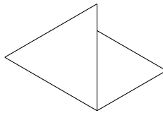
Figure 2.3 Intersections that are not allowed in triangulations
