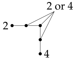
Figure 5.2 Without a 1 in Q_1 , we would have only 2s and 4s, forcing a 24 edge.
