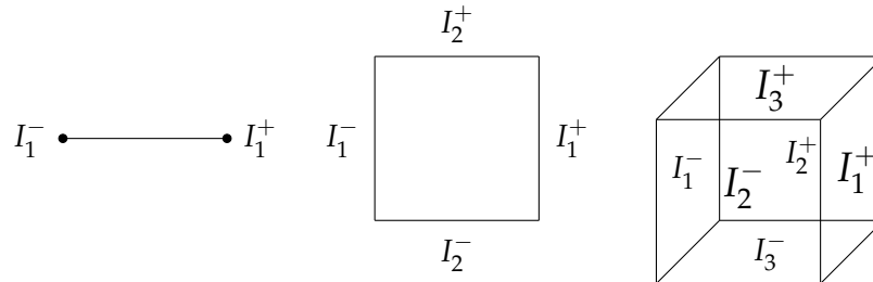
Figure 1.2 The opposite sides of the n -cube for n = 1, 2, 3 .
