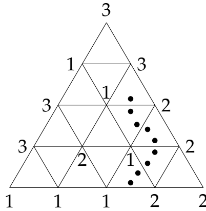
Figure 2.6 Example of a Type 2 Path
