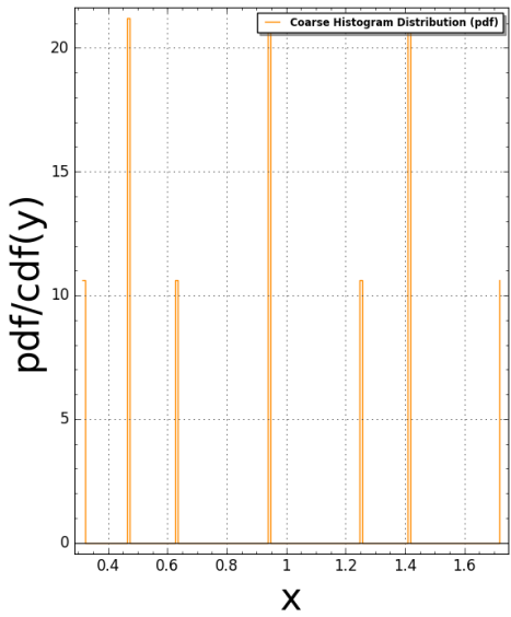
WaltonChair(N:=1) Pair Correlation (Squared): #bins=150, #tiling points = 6 Time Taken: 5.45765 sec (0.0909608 mins)
