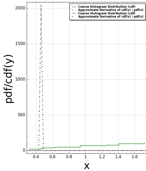
WaltonChair(N:=1) Pair Correlation (Squared): #bins=150, #tiling points = 6 Time Taken: 5.45765 sec (0.0909608 mins)
