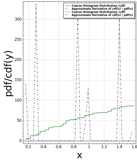
WaltonChair(N:=4) Pair Correlation (Squared): #bins=125, #tiling points = 120 Time Taken: 5.13592 sec (0.0855986 mins)
