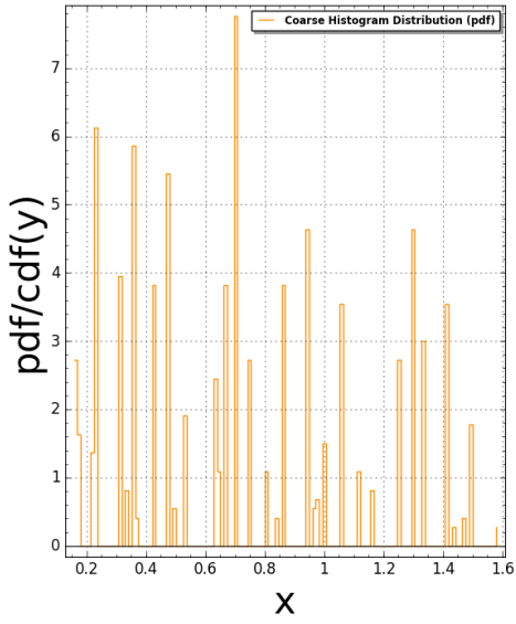
WaltonChair(N:=4) Pair Correlation (Squared): #bins=125, #tiling points = 120 Time Taken: 5.13592 sec (0.0855986 mins)
