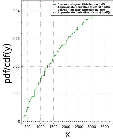
TubingenTriangle(N:=7) Pair Correlation (Squared): #bins=150, #tiling points = 539 Time Taken: 29.7714 sec (0.496189 mins)
