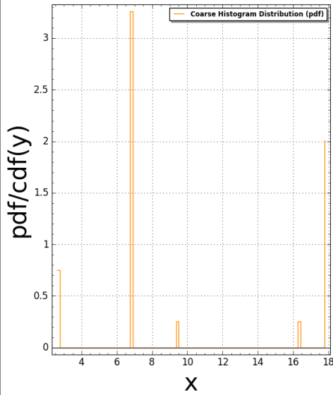
TubingenTriangle(N:=3) Pair Correlation (Squared): #bins=100, #tiling points = 18 Time Taken: 4.02471 sec (0.0670785 mins)
