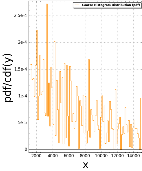
TubingenTriangle(N:=8) Pair Correlation (Squared): #bins=100, #tiling points = 1365 Time Taken: 79.9711 sec (1.33285 mins)
