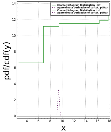
TubingenTriangle(N:=3) Pair Correlation (Squared): #bins=150, #tiling points = 18 Time Taken: 5.16978 sec (0.086163 mins)
