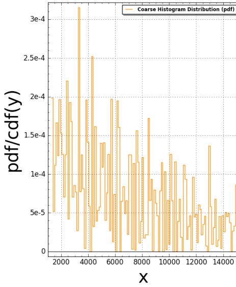
TubingenTriangle(N:=8) Pair Correlation (Squared): #bins=125, #tiling points = 1365 Time Taken: 81.1126 sec (1.35188 mins)
