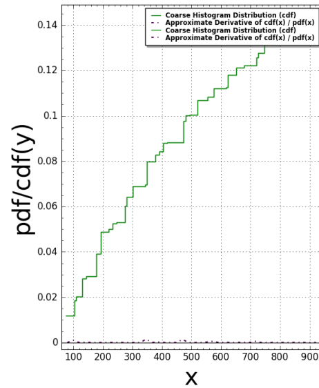
TubingenTriangle(N:=5) Pair Correlation (Squared): #bins=125, #tiling points = 90 Time Taken: 8.22697 sec (0.137116 mins)
