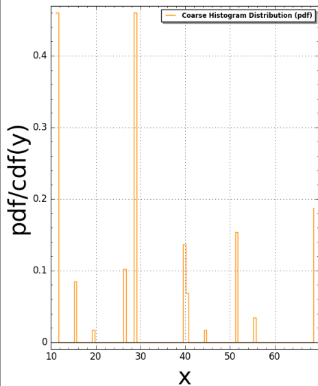
TubingenTriangle(N:=3) Pair Correlation (Squared): #bins=100, #tiling points = 18 Time Taken: 4.02471 sec (0.0670785 mins)
