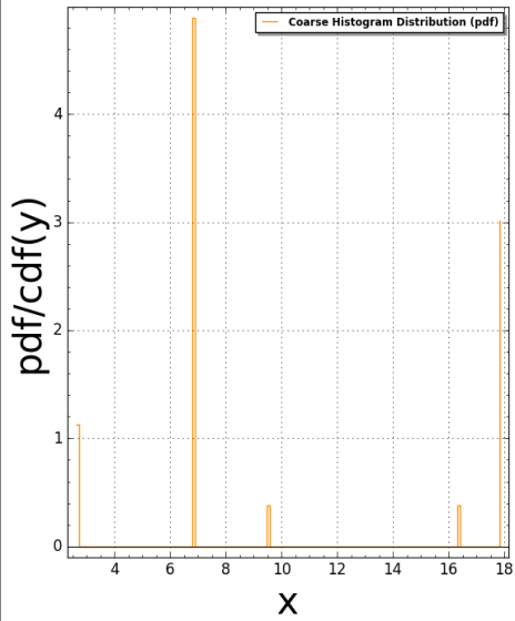
TubingenTriangle(N:=3) Pair Correlation (Squared): #bins=150, #tiling points = 18 Time Taken: 5.16978 sec (0.086163 mins)
