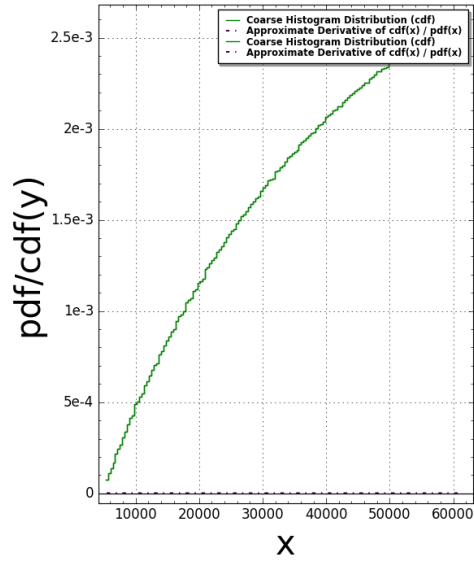
TubingenTriangle(N:=9) Pair Correlation (Squared): #bins=150, #tiling points = 3500 Time Taken: 317.192 sec (5.28654 mins)
