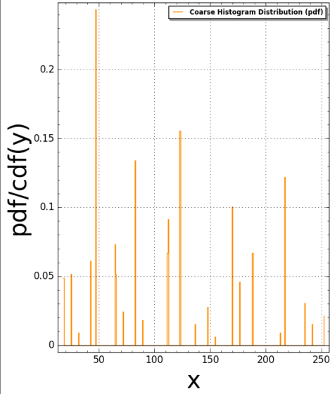
TubingenTriangle(N:=5) Pair Correlation (Squared): #bins=350, #tiling points = 90 Time Taken: 11.2761 sec (0.187935 mins)
