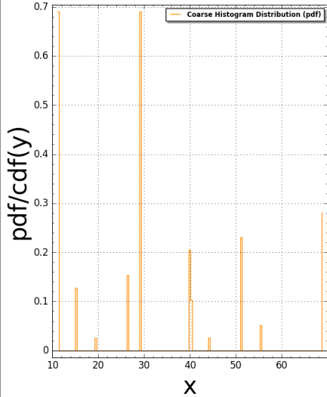
TubingenTriangle(N:=4) Pair Correlation (Squared): #bins=150, #tiling points = 39 Time Taken: 5.72919 sec (0.0954865 mins)
