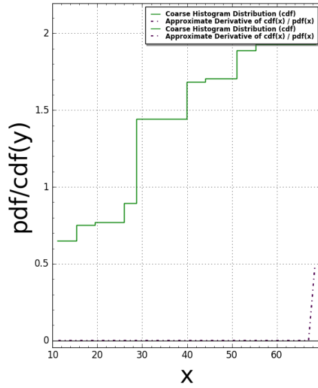
TubingenTriangle(N:=4) Pair Correlation (Squared): #bins=125, #tiling points = 39 Time Taken: 5.19332 sec (0.0865553 mins)
