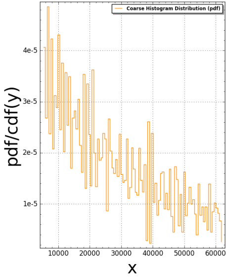
TubingenTriangle(N:=9) Pair Correlation (Squared): #bins=100, #tiling points = 3500 Time Taken: 310.32 sec (5.172 mins)
