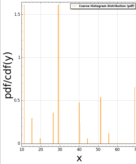
TubingenTriangle(N:=3) Pair Correlation (Squared): #bins=350, #tiling points = 18 Time Taken: 7.1278 sec (0.118797 mins)
