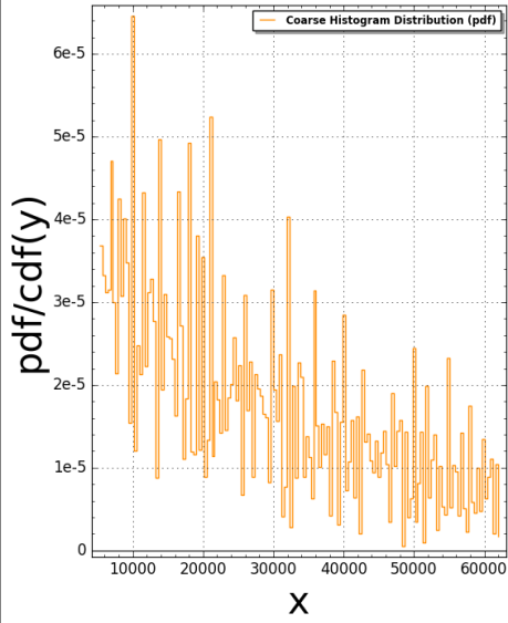
TubingenTriangle(N:=9) Pair Correlation (Squared): #bins=150, #tiling points = 3500 Time Taken: 317.192 sec (5.28654 mins)
