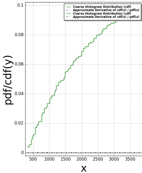
TubingenTriangle(N:=6) Pair Correlation (Squared): #bins=350, #tiling points = 217 Time Taken: 16.0525 sec (0.267542 mins)
