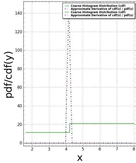
TubingenTriangle(N:=2) Pair Correlation (Squared): #bins=100, #tiling points = 9 Time Taken: 4.02288 sec (0.067048 mins)
