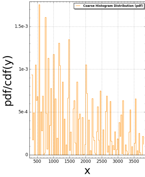
TubingenTriangle(N:=7) Pair Correlation (Squared): #bins=125, #tiling points = 539 Time Taken: 28.9945 sec (0.483241 mins)
