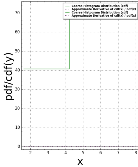
TubingenTriangle(N:=2) Pair Correlation (Squared): #bins=350, #tiling points = 9 Time Taken: 7.21806 sec (0.120301 mins)
