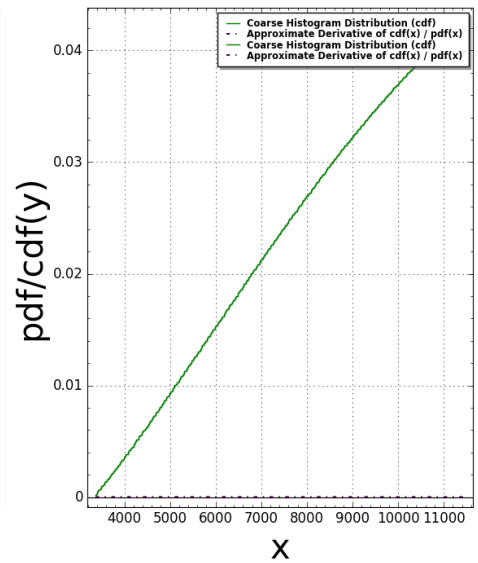
TubingenTriangle(N:=11) Pair Correlation: #bins=350, #tiling points = 23490 Time Taken: 10786.9 sec (179.781 mins)
