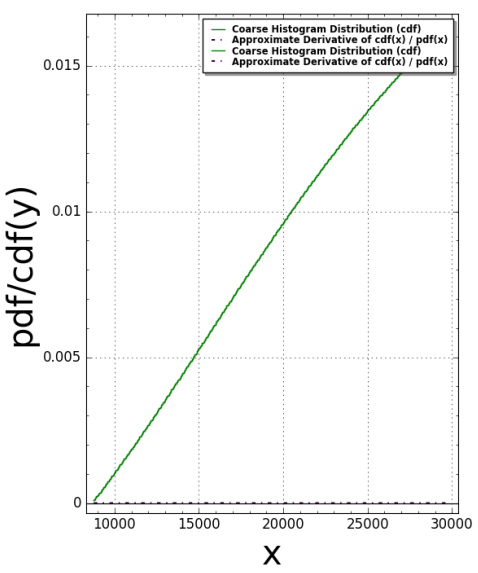
TubingenTriangle(N:=11) Pair Correlation: #bins=350, #tiling points = 23490 Time Taken: 10786.9 sec (179.781 mins)
