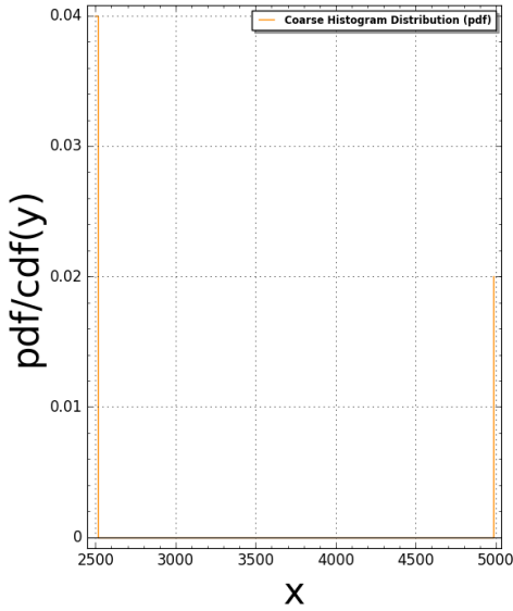
Tetris(N:=1) Pair Correlation (Squared): #bins=150, #tiling points = 4 Time Taken: 4.8137 sec (0.0802283 mins)
