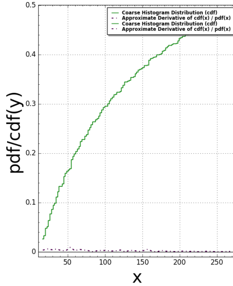
T2000Triangle(N:=1) Pair Correlation (Squared): #bins=150, #tiling points = 3 Time Taken: 4.57876 sec (0.0763126 mins)
