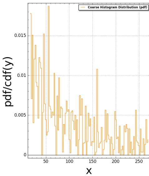
T2000Triangle(N:=1) Pair Correlation (Squared): #bins=150, #tiling points = 3 Time Taken: 4.57876 sec (0.0763126 mins)
