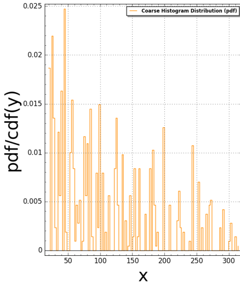
T2000Triangle(N:=7) Pair Correlation (Squared): #bins=125, #tiling points = 206 Time Taken: 7.24994 sec (0.120832 mins)
