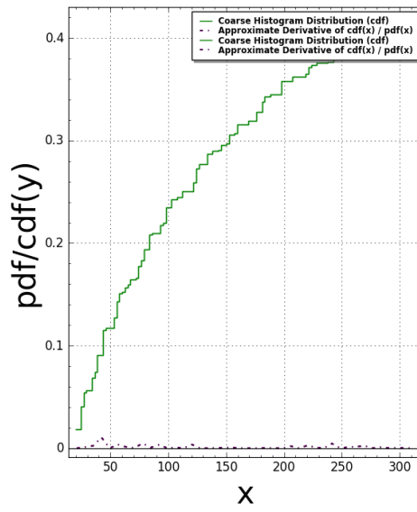
T2000Triangle(N:=7) Pair Correlation (Squared): #bins=125, #tiling points = 206 Time Taken: 7.24994 sec (0.120832 mins)
