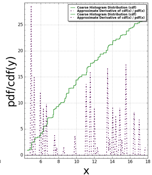
T2000Triangle(N:=6) Pair Correlation: #bins=350, #tiling points = 75 Time Taken: 7.97012 sec (0.132835 mins)
