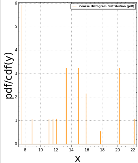
T2000Triangle(N:=4) Pair Correlation: #bins=350, #tiling points = 12 Time Taken: 7.02916 sec (0.117153 mins)
