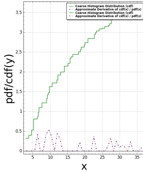
Sphinx(N:=5) Pair Correlation (Squared): #bins=125, #tiling points = 638 Time Taken: 10.833 sec (0.18055 mins)
