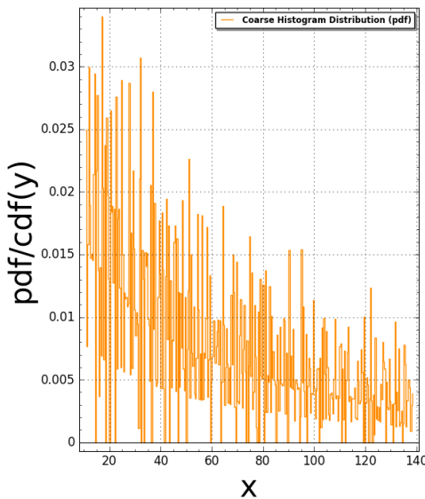
Sphinx(N:=6) Pair Correlation (Squared): #bins=350, #tiling points = 2555 Time Taken: 96.2518 sec (1.6042 mins)
