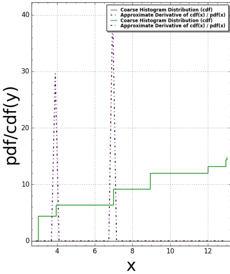
Sphinx(N:=3) Pair Correlation (Squared): #bins=150, #tiling points = 39 Time Taken: 6.2781 sec (0.104635 mins)
