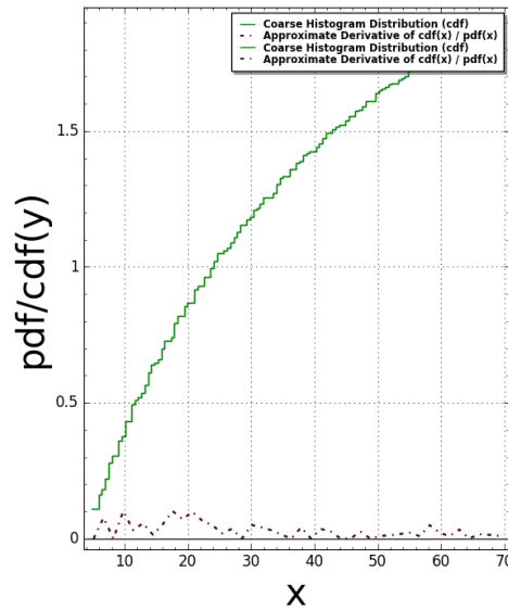
Sphinx(N:=6) Pair Correlation (Squared): #bins=125, #tiling points = 2555 Time Taken: 72.8709 sec (1.21451 mins)
