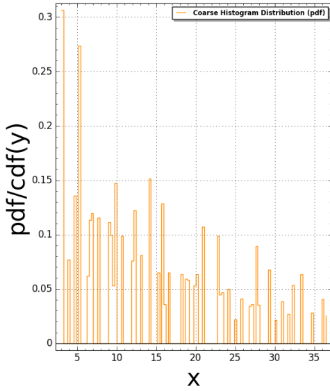
Sphinx(N:=5) Pair Correlation (Squared): #bins=125, #tiling points = 638 Time Taken: 10.833 sec (0.18055 mins)
