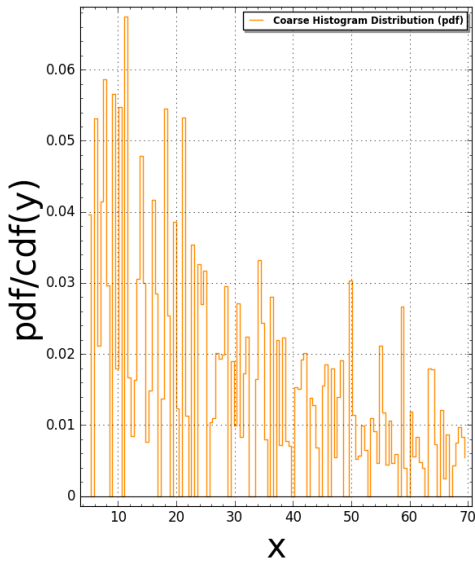
Sphinx(N:=6) Pair Correlation (Squared): #bins=125, #tiling points = 2555 Time Taken: 72.8709 sec (1.21451 mins)
