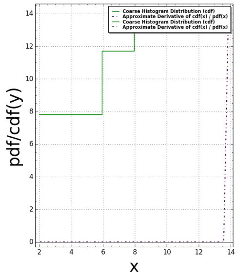
Sphinx(N:=1) Pair Correlation (Squared): #bins=125, #tiling points = 5 Time Taken: 6.18337 sec (0.103056 mins)
