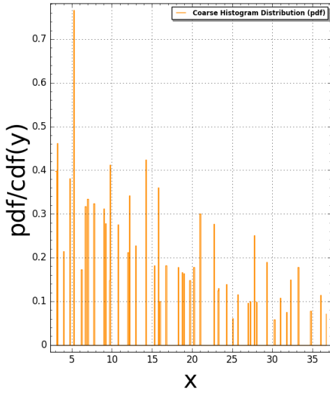
Sphinx(N:=5) Pair Correlation (Squared): #bins=350, #tiling points = 638 Time Taken: 14.4194 sec (0.240324 mins)
