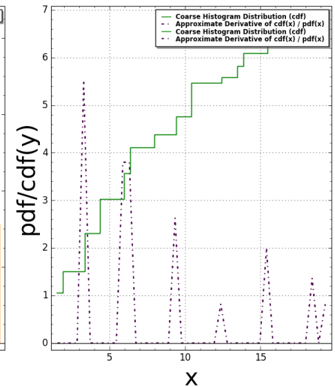
Sphinx(N:=3) Pair Correlation (Squared): #bins=125, #tiling points = 39 Time Taken: 5.68137 sec (0.0946896 mins)
