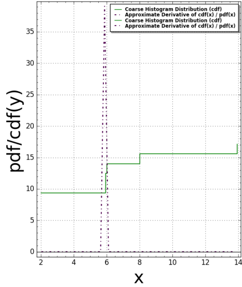
Sphinx(N:=2) Pair Correlation (Squared): #bins=150, #tiling points = 11 Time Taken: 6.92821 sec (0.11547 mins)
