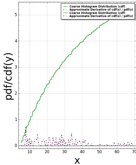
Sphinx(N:=6) Pair Correlation (Squared): #bins=350, #tiling points = 2555 Time Taken: 96.2518 sec (1.6042 mins)
