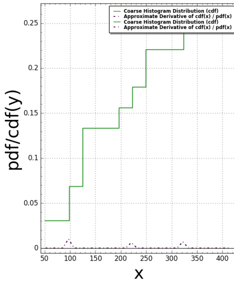
Pentomino(N:=3) Pair Correlation (Squared): #bins=100, #tiling points = 49 Time Taken: 4.10512 sec (0.0684187 mins)
