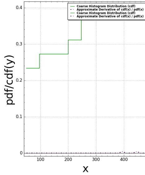
Pentomino(N:=2) Pair Correlation (Squared): #bins=100, #tiling points = 15 Time Taken: 3.6847 sec (0.0614117 mins)
