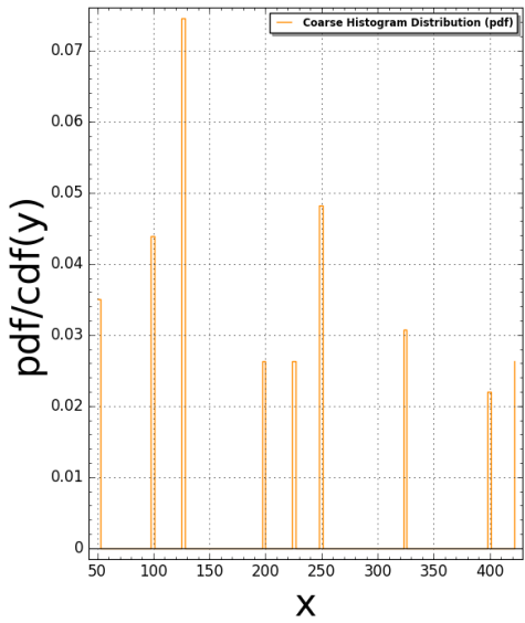
Pentomino(N:=2) Pair Correlation (Squared): #bins=125, #tiling points = 15 Time Taken: 4.30536 sec (0.071756 mins)
