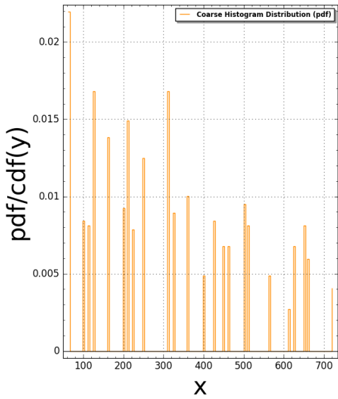
Pentomino(N:=4) Pair Correlation (Squared): #bins=150, #tiling points = 183 Time Taken: 5.66811 sec (0.0944685 mins)
