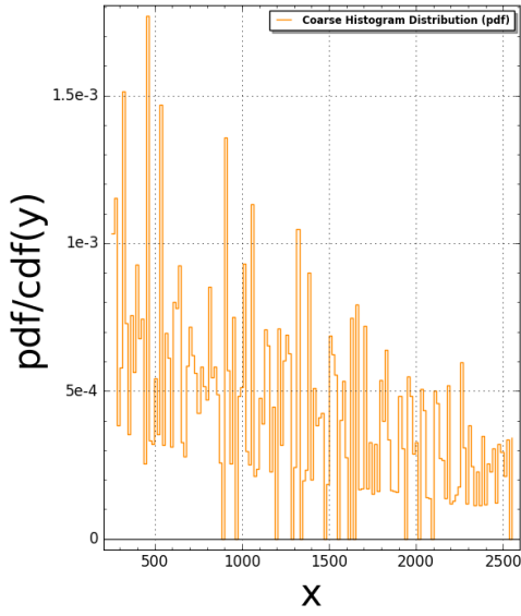
Pentomino(N:=6) Pair Correlation (Squared): #bins=150, #tiling points = 2802 Time Taken: 54.4237 sec (0.907062 mins)
