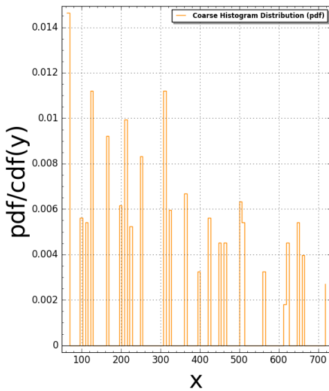
Pentomino(N:=3) Pair Correlation (Squared): #bins=100, #tiling points = 49 Time Taken: 4.10512 sec (0.0684187 mins)
