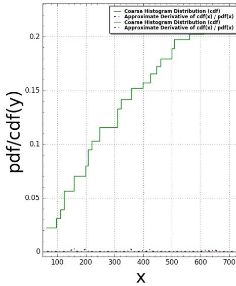
Pentomino(N:=4) Pair Correlation (Squared): #bins=150, #tiling points = 183 Time Taken: 5.66811 sec (0.0944685 mins)
