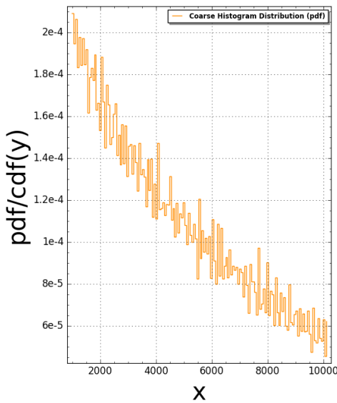
Pentomino(N:=7) Pair Correlation (Squared): #bins=150, #tiling points = 11135 Time Taken: 615.1 sec (10.2517 mins)
