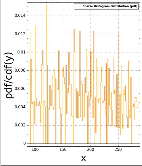
Pentomino(N:=6) Pair Correlation: #bins=150, #tiling points = 2802 Time Taken: 56.0437 sec (0.934062 mins)
