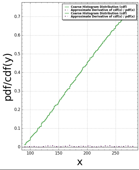
Pentomino(N:=6) Pair Correlation: #bins=150, #tiling points = 2802 Time Taken: 56.0437 sec (0.934062 mins)
