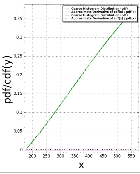
Pentomino(N:=7) Pair Correlation: #bins=150, #tiling points = 11135 Time Taken: 617.466 sec (10.2911 mins)
