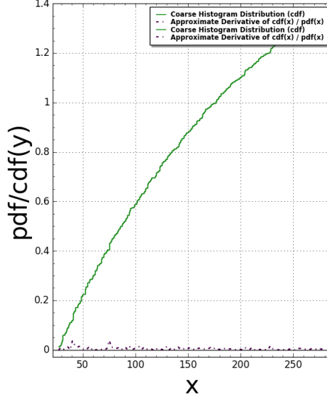
Pentagon5(N:=5) Pair Correlation (Squared): #bins=350, #tiling points = 1365 Time Taken: 26.2361 sec (0.437268 mins)
