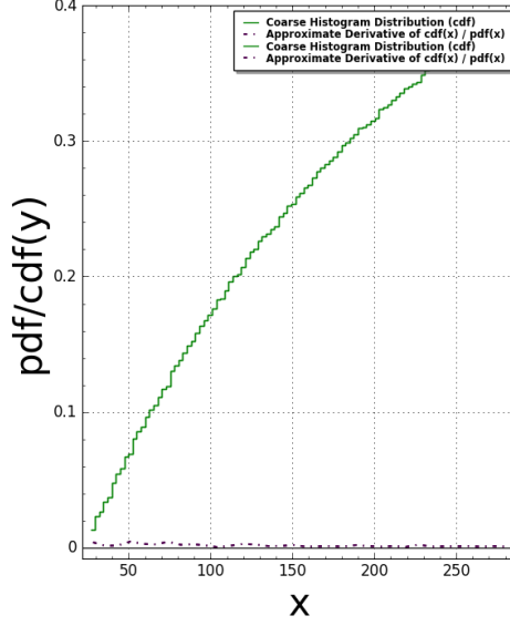
Pentagon5(N:=5) Pair Correlation (Squared): #bins=100, #tiling points = 1365 Time Taken: 20.5926 sec (0.34321 mins)
