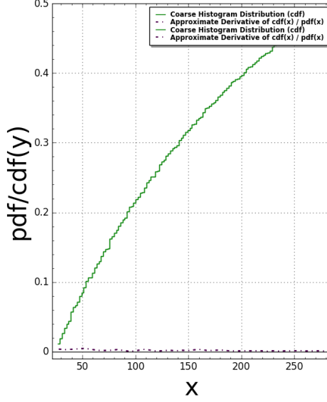
Pentagon5(N:=5) Pair Correlation (Squared): #bins=125, #tiling points = 1365 Time Taken: 21.825 sec (0.36375 mins)
