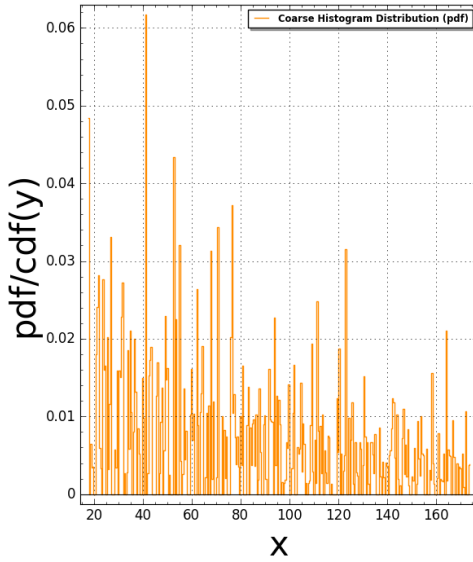
Pentagon5(N:=3) Pair Correlation (Squared): #bins=350, #tiling points = 565 Time Taken: 12.8203 sec (0.213672 mins)
