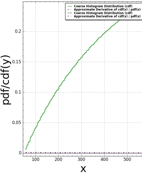
Pentagon5(N:=6) Pair Correlation (Squared): #bins=125, #tiling points = 1845 Time Taken: 31.1501 sec (0.519169 mins)
