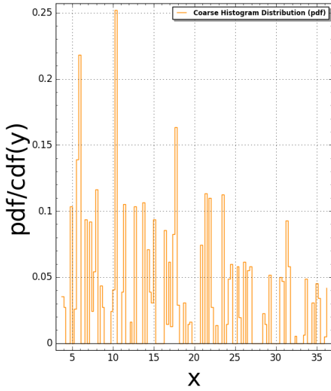
Pentagon5(N:=2) Pair Correlation (Squared): #bins=125, #tiling points = 309 Time Taken: 6.79972 sec (0.113329 mins)
