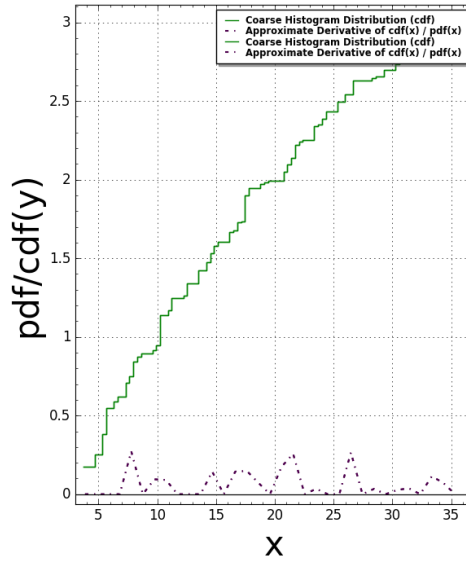
Pentagon5(N:=2) Pair Correlation (Squared): #bins=100, #tiling points = 309 Time Taken: 6.11496 sec (0.101916 mins)
