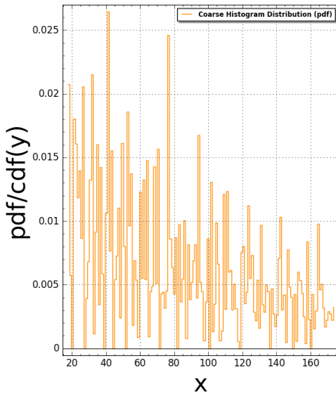
Pentagon5(N:=3) Pair Correlation (Squared): #bins=150, #tiling points = 565 Time Taken: 10.5816 sec (0.176361 mins)
