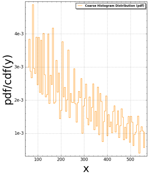
Pentagon5(N:=6) Pair Correlation (Squared): #bins=100, #tiling points = 1845 Time Taken: 29.6522 sec (0.494204 mins)
