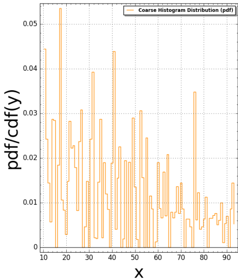
Pentagon5(N:=3) Pair Correlation (Squared): #bins=100, #tiling points = 565 Time Taken: 9.13591 sec (0.152265 mins)
