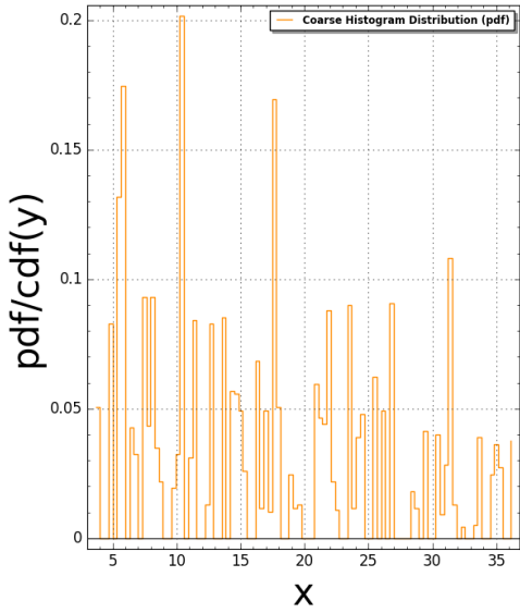
Pentagon5(N:=2) Pair Correlation (Squared): #bins=100, #tiling points = 309 Time Taken: 6.11496 sec (0.101916 mins)
