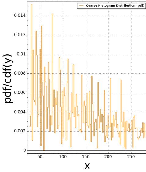
Pentagon5(N:=5) Pair Correlation (Squared): #bins=150, #tiling points = 1365 Time Taken: 22.9275 sec (0.382124 mins)
