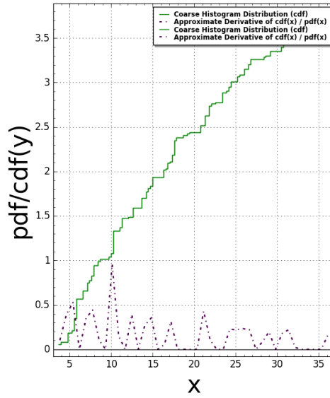
Pentagon5(N:=2) Pair Correlation (Squared): #bins=125, #tiling points = 309 Time Taken: 6.79972 sec (0.113329 mins)
