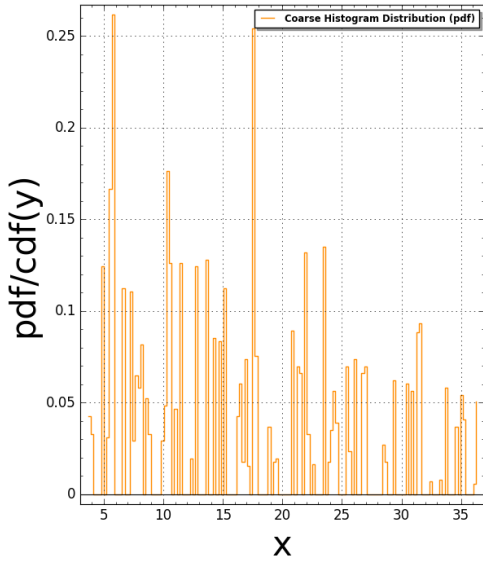
Pentagon5(N:=2) Pair Correlation (Squared): #bins=150, #tiling points = 309 Time Taken: 7.62369 sec (0.127061 mins)
