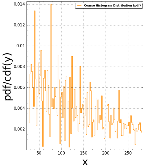
Pentagon5(N:=5) Pair Correlation (Squared): #bins=125, #tiling points = 1365 Time Taken: 21.825 sec (0.36375 mins)
