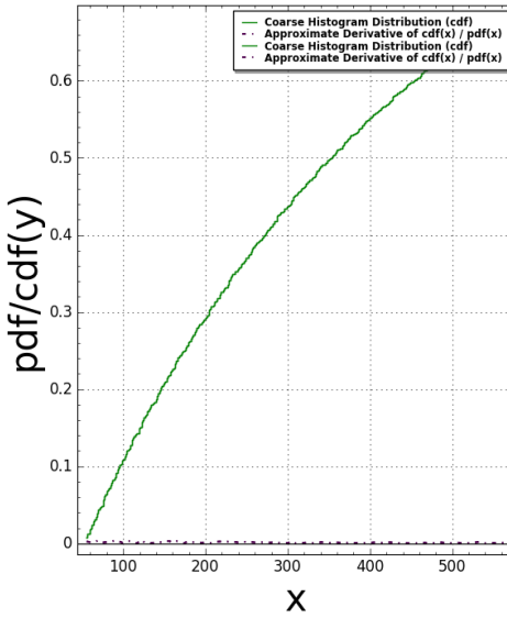
Pentagon5(N:=6) Pair Correlation (Squared): #bins=350, #tiling points = 1845 Time Taken: 36.7881 sec (0.613135 mins)
