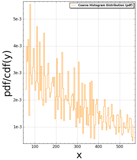
Pentagon5(N:=6) Pair Correlation (Squared): #bins=125, #tiling points = 1845 Time Taken: 31.1501 sec (0.519169 mins)
