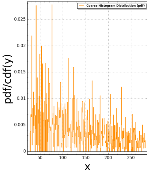
Pentagon5(N:=5) Pair Correlation (Squared): #bins=350, #tiling points = 1365 Time Taken: 26.2361 sec (0.437268 mins)
