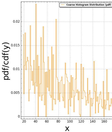
Pentagon5(N:=3) Pair Correlation (Squared): #bins=125, #tiling points = 565 Time Taken: 9.83767 sec (0.163961 mins)
