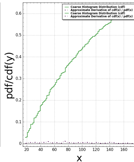
Pentagon5(N:=3) Pair Correlation (Squared): #bins=100, #tiling points = 565 Time Taken: 9.13591 sec (0.152265 mins)
