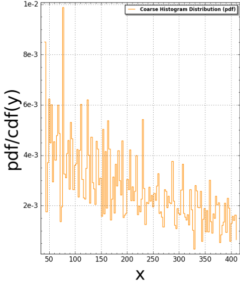
Pentagon5(N:=6) Pair Correlation (Squared): #bins=150, #tiling points = 1845 Time Taken: 32.4844 sec (0.541407 mins)
