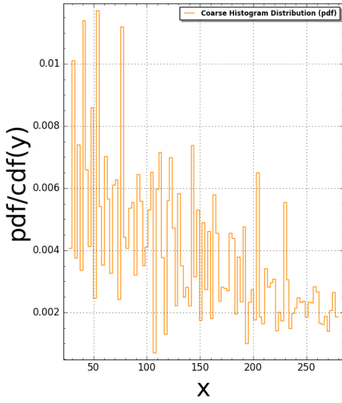
Pentagon5(N:=5) Pair Correlation (Squared): #bins=100, #tiling points = 1365 Time Taken: 20.5926 sec (0.34321 mins)
