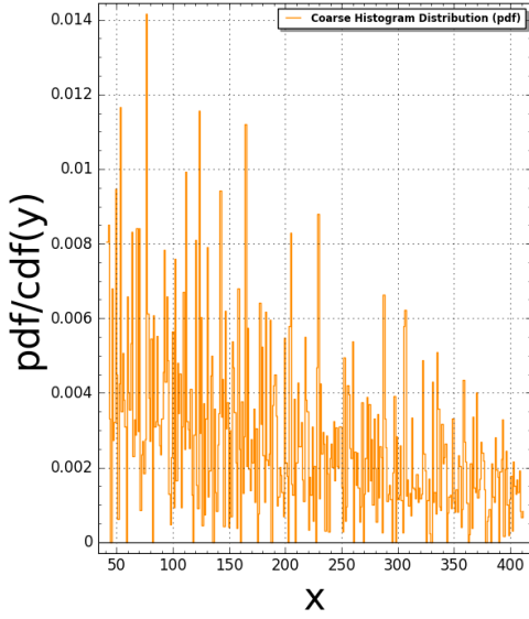
Pentagon5(N:=6) Pair Correlation (Squared): #bins=350, #tiling points = 1845 Time Taken: 36.7881 sec (0.613135 mins)
