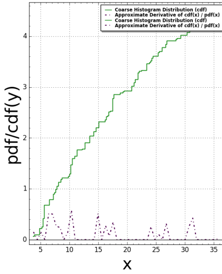
Pentagon5(N:=2) Pair Correlation (Squared): #bins=150, #tiling points = 309 Time Taken: 7.62369 sec (0.127061 mins)
