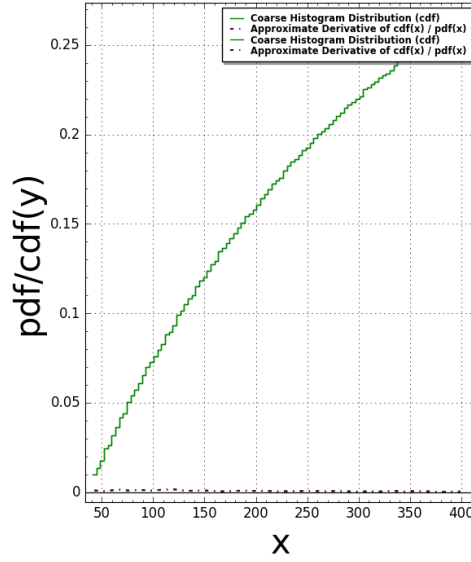
Pentagon5(N:=6) Pair Correlation (Squared): #bins=100, #tiling points = 1845 Time Taken: 29.6522 sec (0.494204 mins)
