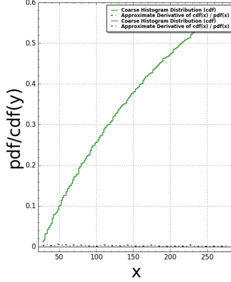
Pentagon5(N:=5) Pair Correlation (Squared): #bins=150, #tiling points = 1365 Time Taken: 22.9275 sec (0.382124 mins)
