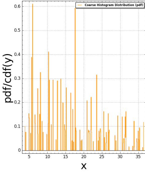
Pentagon5(N:=2) Pair Correlation (Squared): #bins=350, #tiling points = 309 Time Taken: 9.79457 sec (0.163243 mins)
