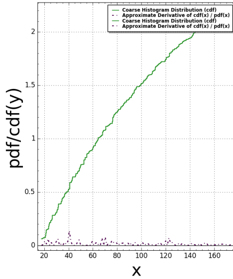
Pentagon5(N:=3) Pair Correlation (Squared): #bins=350, #tiling points = 565 Time Taken: 12.8203 sec (0.213672 mins)
