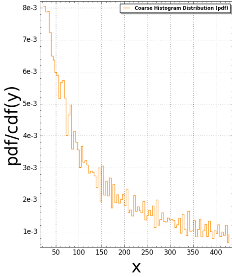
Pentagon15(N:=5) Pair Correlation (Squared): #bins=100, #tiling points = 2754 Time Taken: 51.4341 sec (0.857235 mins)
