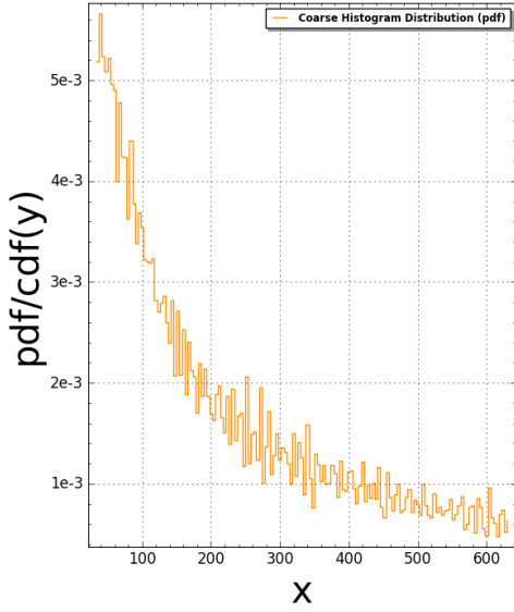
Pentagon15(N:=6) Pair Correlation (Squared): #bins=150, #tiling points = 3778 Time Taken: 92.2052 sec (1.53675 mins)
