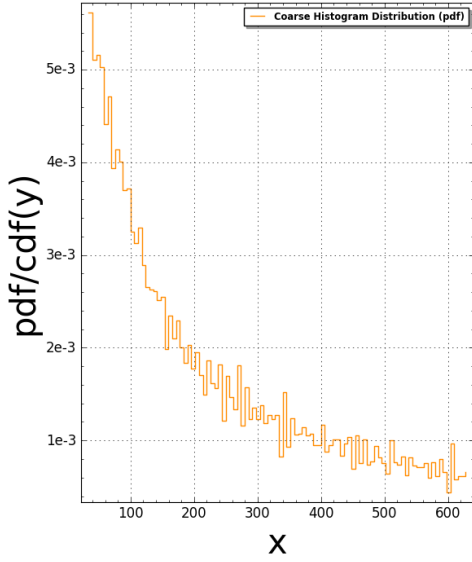
Pentagon15(N:=6) Pair Correlation (Squared): #bins=100, #tiling points = 3778 Time Taken: 84.1699 sec (1.40283 mins)
