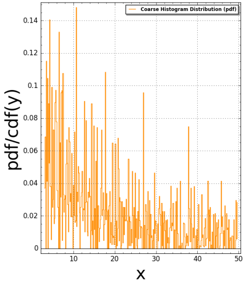
Pentagon15(N:=2) Pair Correlation (Squared): #bins=350, #tiling points = 610 Time Taken: 11.9589 sec (0.199315 mins)
