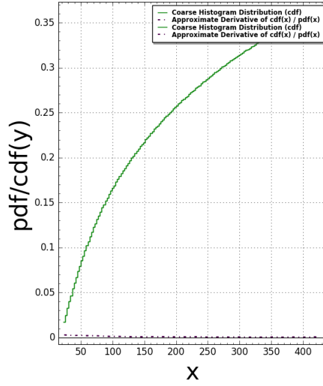
Pentagon15(N:=5) Pair Correlation (Squared): #bins=150, #tiling points = 2754 Time Taken: 56.0875 sec (0.934791 mins)
