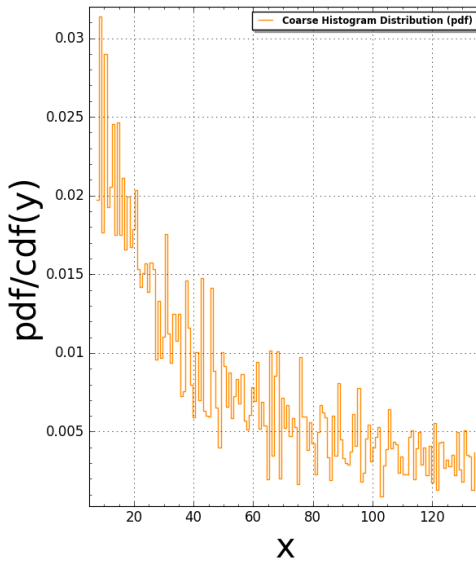
Pentagon15(N:=3) Pair Correlation (Squared): #bins=150, #tiling points = 1162 Time Taken: 17.9015 sec (0.298358 mins)
