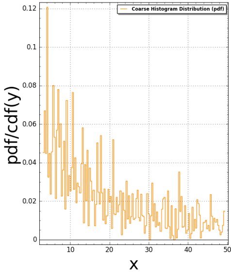
Pentagon15(N:=2) Pair Correlation (Squared): #bins=150, #tiling points = 610 Time Taken: 9.86228 sec (0.164371 mins)
