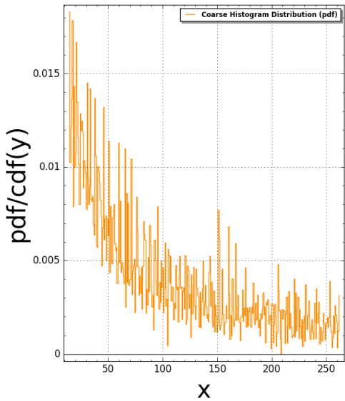
Pentagon15(N:=3) Pair Correlation (Squared): #bins=350, #tiling points = 1162 Time Taken: 20.784 sec (0.3464 mins)
