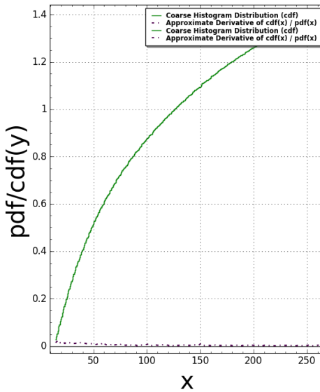
Pentagon15(N:=3) Pair Correlation (Squared): #bins=350, #tiling points = 1162 Time Taken: 20.784 sec (0.3464 mins)
