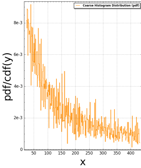
Pentagon15(N:=5) Pair Correlation (Squared): #bins=350, #tiling points = 2754 Time Taken: 63.1517 sec (1.05253 mins)
