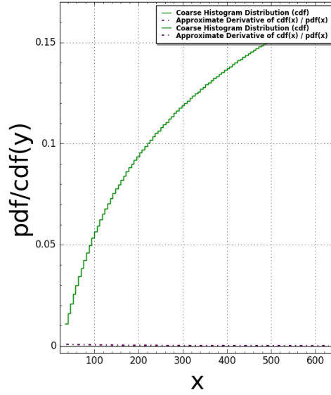
Pentagon15(N:=6) Pair Correlation (Squared): #bins=100, #tiling points = 3778 Time Taken: 84.1699 sec (1.40283 mins)
