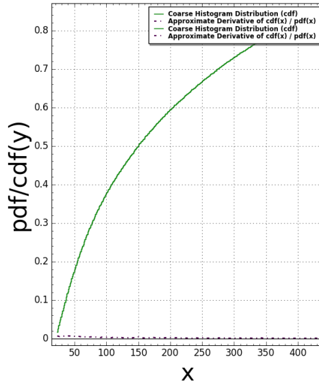
Pentagon15(N:=5) Pair Correlation (Squared): #bins=350, #tiling points = 2754 Time Taken: 63.1517 sec (1.05253 mins)
