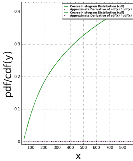
Pentagon15(N:=6) Pair Correlation (Squared): #bins=350, #tiling points = 3778 Time Taken: 105.382 sec (1.75637 mins)
