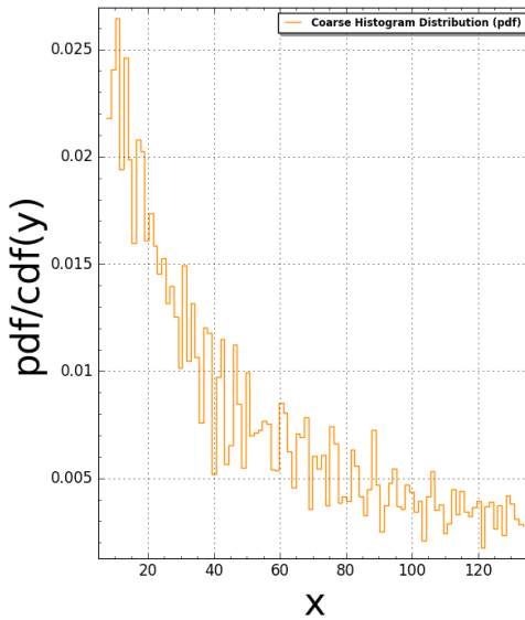
Pentagon15(N:=3) Pair Correlation (Squared): #bins=100, #tiling points = 1162 Time Taken: 16.0301 sec (0.267168 mins)
