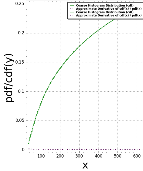
Pentagon15(N:=6) Pair Correlation (Squared): #bins=150, #tiling points = 3778 Time Taken: 92.2052 sec (1.53675 mins)
