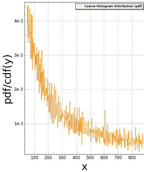
Pentagon15(N:=6) Pair Correlation (Squared): #bins=350, #tiling points = 3778 Time Taken: 105.382 sec (1.75637 mins)
