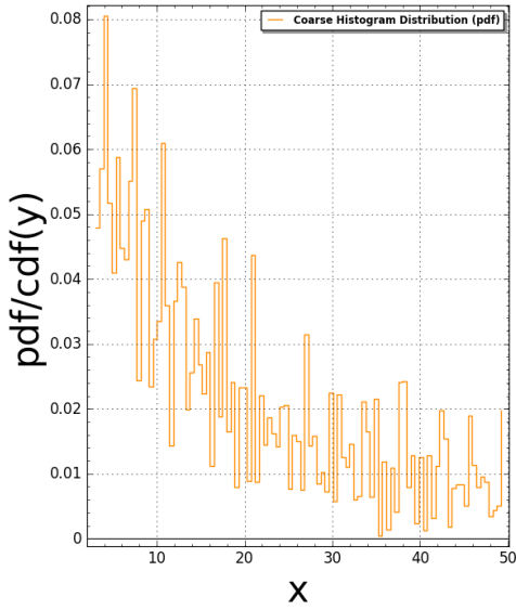
Pentagon15(N:=2) Pair Correlation (Squared): #bins=100, #tiling points = 610 Time Taken: 8.54679 sec (0.142447 mins)
