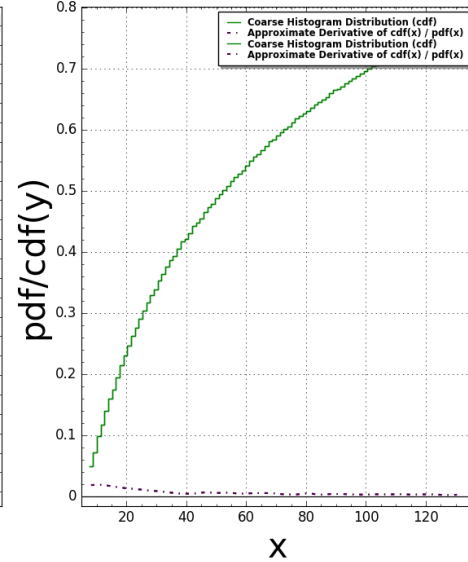
Pentagon15(N:=3) Pair Correlation (Squared): #bins=100, #tiling points = 1162 Time Taken: 16.0301 sec (0.267168 mins)
