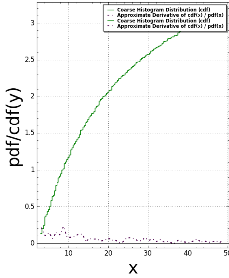
Pentagon15(N:=2) Pair Correlation (Squared): #bins=150, #tiling points = 610 Time Taken: 9.86228 sec (0.164371 mins)
