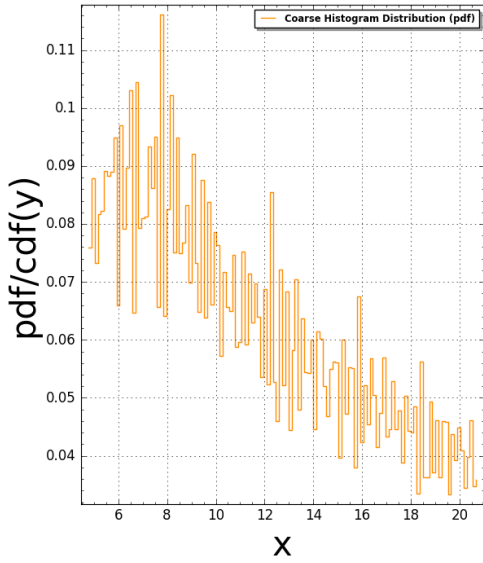
Pentagon15(N:=5) Pair Correlation: #bins=125, #tiling points = 2754 Time Taken: 53.5183 sec (0.891972 mins)
