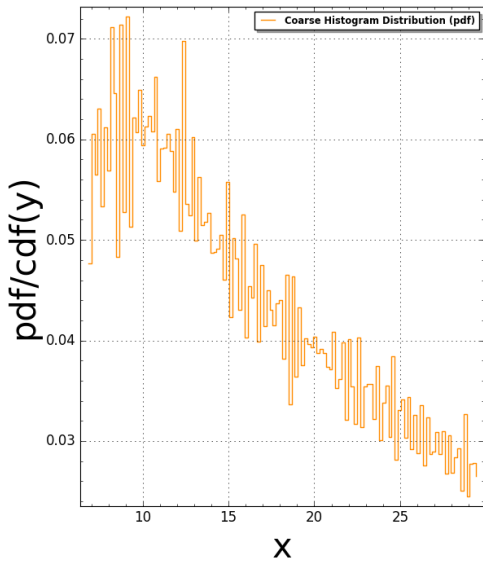
Pentagon15(N:=6) Pair Correlation: #bins=125, #tiling points = 3778 Time Taken: 88.7107 sec (1.47851 mins)
