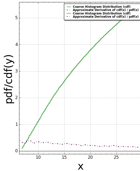
Pentagon15(N:=6) Pair Correlation: #bins=125, #tiling points = 3778 Time Taken: 88.7107 sec (1.47851 mins)
