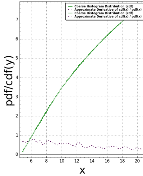
Pentagon15(N:=5) Pair Correlation: #bins=125, #tiling points = 2754 Time Taken: 53.5183 sec (0.891972 mins)
