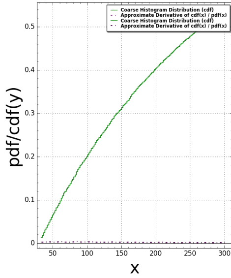
Pentagon11(N:=5) Pair Correlation (Squared): #bins=150, #tiling points = 2371 Time Taken: 41.7601 sec (0.696001 mins)
