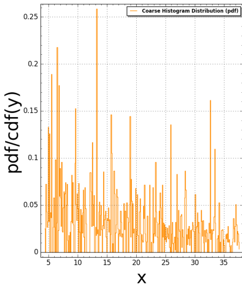
Pentagon11(N:=2) Pair Correlation (Squared): #bins=350, #tiling points = 516 Time Taken: 10.5034 sec (0.175056 mins)
