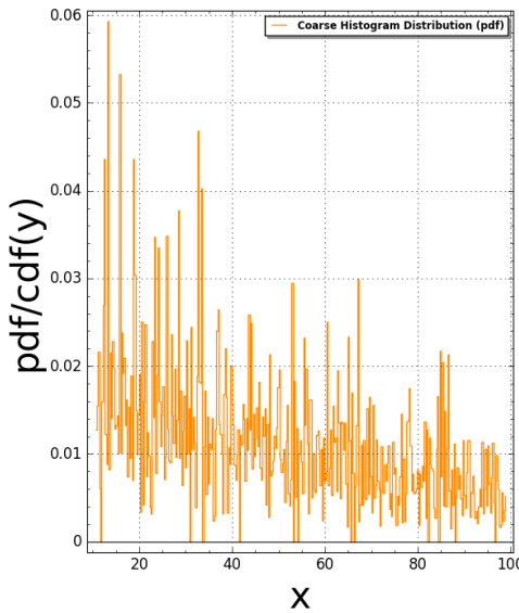
Pentagon11(N:=3) Pair Correlation (Squared): #bins=350, #tiling points = 1002 Time Taken: 16.341 sec (0.272351 mins)
