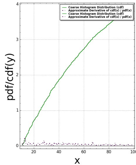
Pentagon11(N:=3) Pair Correlation (Squared): #bins=350, #tiling points = 1002 Time Taken: 16.341 sec (0.272351 mins)
