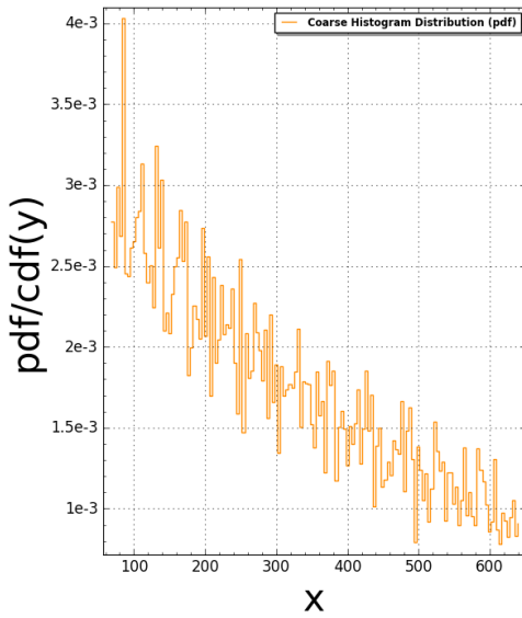
Pentagon11(N:=6) Pair Correlation (Squared): #bins=150, #tiling points = 3345 Time Taken: 73.0872 sec (1.21812 mins)
