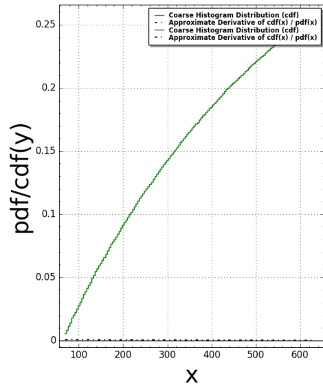
Pentagon11(N:=6) Pair Correlation (Squared): #bins=150, #tiling points = 3345 Time Taken: 73.0872 sec (1.21812 mins)
