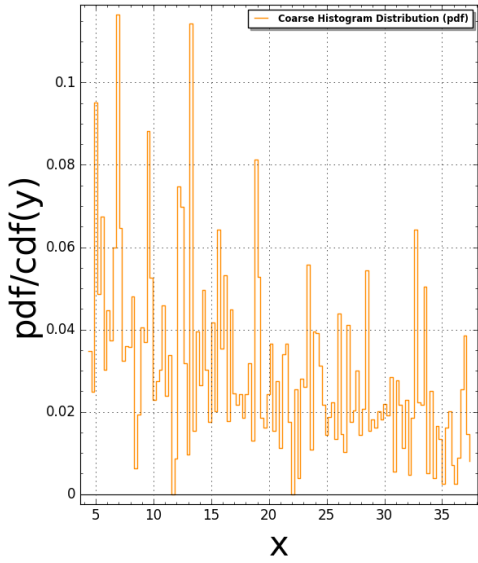
Pentagon11(N:=2) Pair Correlation (Squared): #bins=125, #tiling points = 516 Time Taken: 7.94178 sec (0.132363 mins)
