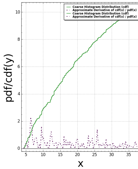
Pentagon11(N:=2) Pair Correlation (Squared): #bins=350, #tiling points = 516 Time Taken: 10.5034 sec (0.175056 mins)
