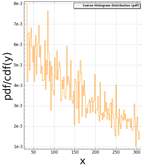
Pentagon11(N:=5) Pair Correlation (Squared): #bins=150, #tiling points = 2371 Time Taken: 41.7601 sec (0.696001 mins)
