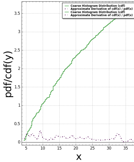
Pentagon11(N:=2) Pair Correlation (Squared): #bins=125, #tiling points = 516 Time Taken: 7.94178 sec (0.132363 mins)
