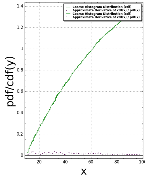
Pentagon11(N:=3) Pair Correlation (Squared): #bins=125, #tiling points = 1002 Time Taken: 13.1291 sec (0.218818 mins)
