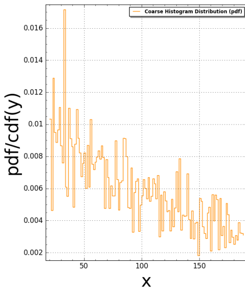
Pentagon11(N:=3) Pair Correlation (Squared): #bins=125, #tiling points = 1002 Time Taken: 13.1291 sec (0.218818 mins)
