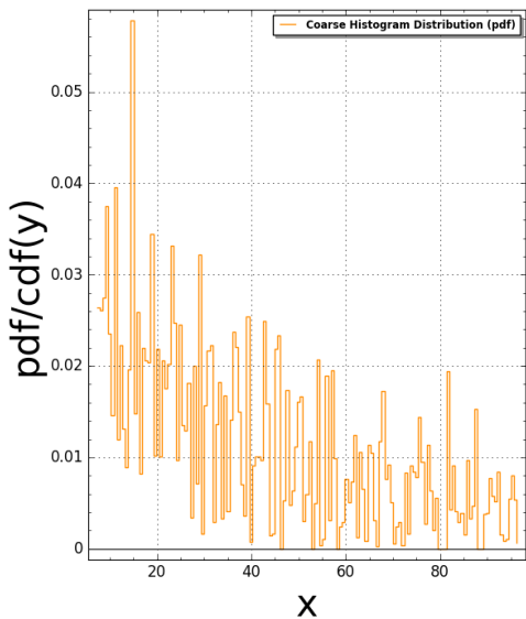
Pentagon1(N:=3) Pair Correlation (Squared): #bins=150, #tiling points = 224 Time Taken: 6.3446 sec (0.105743 mins)
