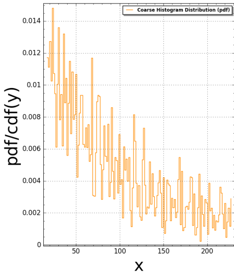
Pentagon1(N:=6) Pair Correlation (Squared): #bins=150, #tiling points = 728 Time Taken: 11.6739 sec (0.194566 mins)
