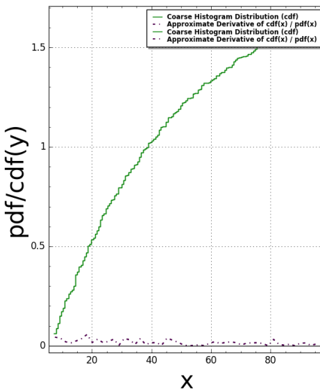
Pentagon1(N:=3) Pair Correlation (Squared): #bins=150, #tiling points = 224 Time Taken: 6.3446 sec (0.105743 mins)
