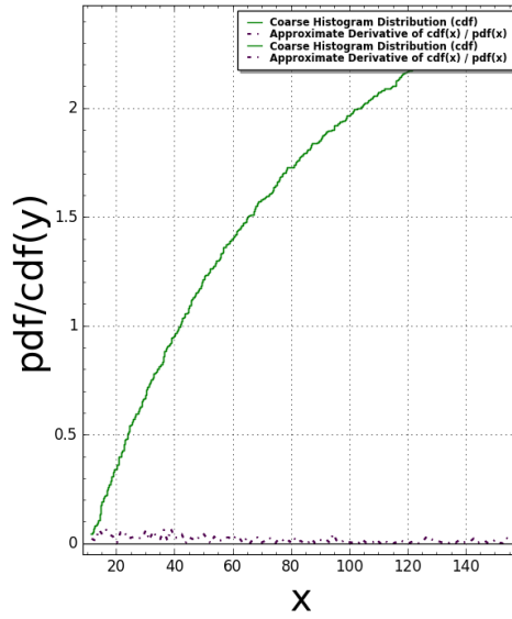
Pentagon1(N:=5) Pair Correlation (Squared): #bins=350, #tiling points = 528 Time Taken: 10.9453 sec (0.182422 mins)
