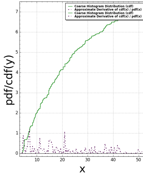
Pentagon1(N:=3) Pair Correlation (Squared): #bins=350, #tiling points = 224 Time Taken: 8.10198 sec (0.135033 mins)
