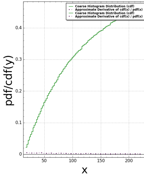
Pentagon1(N:=6) Pair Correlation (Squared): #bins=100, #tiling points = 728 Time Taken: 10.1626 sec (0.169377 mins)
