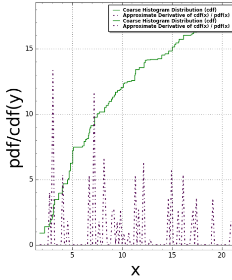
Pentagon1(N:=2) Pair Correlation (Squared): #bins=350, #tiling points = 120 Time Taken: 7.42381 sec (0.12373 mins)
