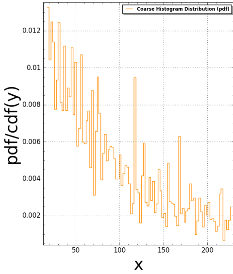
Pentagon1(N:=6) Pair Correlation (Squared): #bins=100, #tiling points = 728 Time Taken: 10.1626 sec (0.169377 mins)
