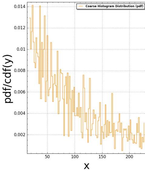
Pentagon1(N:=6) Pair Correlation (Squared): #bins=125, #tiling points = 728 Time Taken: 10.9875 sec (0.183125 mins)
