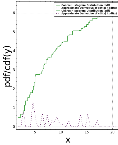
Pentagon1(N:=2) Pair Correlation (Squared): #bins=125, #tiling points = 120 Time Taken: 4.91547 sec (0.0819245 mins)
