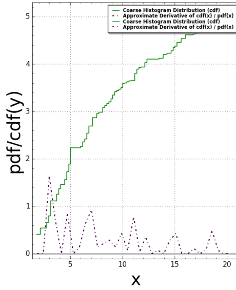
Pentagon1(N:=2) Pair Correlation (Squared): #bins=100, #tiling points = 120 Time Taken: 4.34302 sec (0.0723836 mins)
