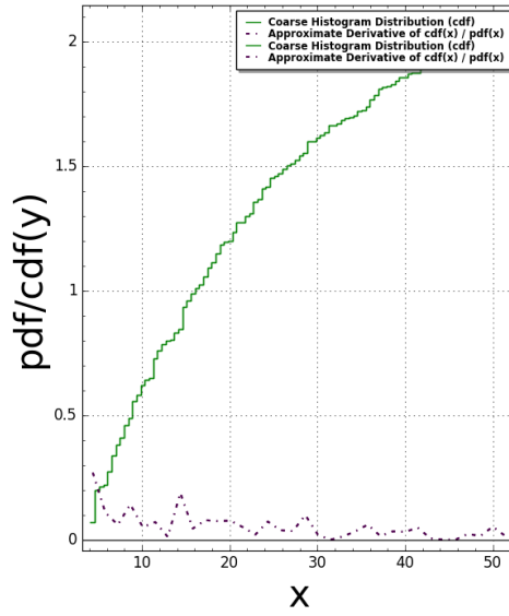
Pentagon1(N:=3) Pair Correlation (Squared): #bins=100, #tiling points = 224 Time Taken: 5.12696 sec (0.0854493 mins)
