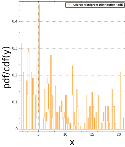
Pentagon1(N:=2) Pair Correlation (Squared): #bins=150, #tiling points = 120 Time Taken: 5.52887 sec (0.0921478 mins)
