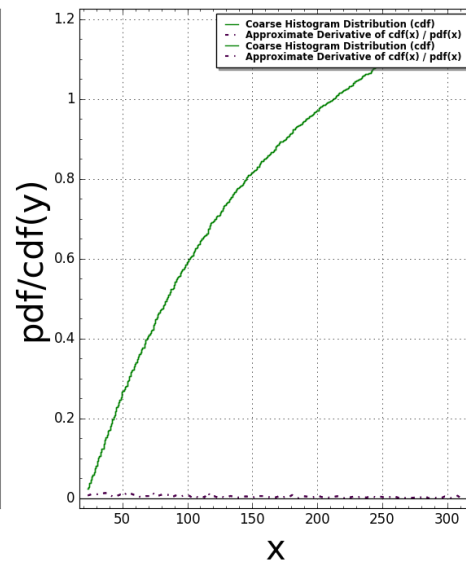
Pentagon1(N:=6) Pair Correlation (Squared): #bins=350, #tiling points = 728 Time Taken: 14.0139 sec (0.233565 mins)
