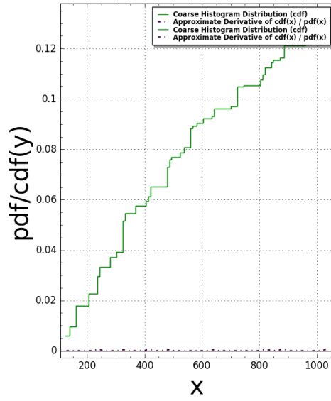
Octagonal1225(N:=4) Pair Correlation (Squared): #bins=125, #tiling points = 152 Time Taken: 5.41387 sec (0.0902312 mins)
