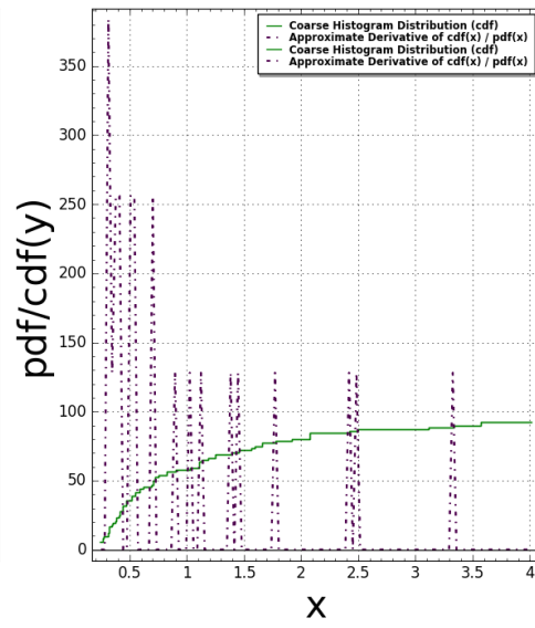
MiniTangram(N:=6) Slope Gaps: #bins=350, #tiling points = 353 Time Taken: 9.9961 sec (0.166602 mins)
