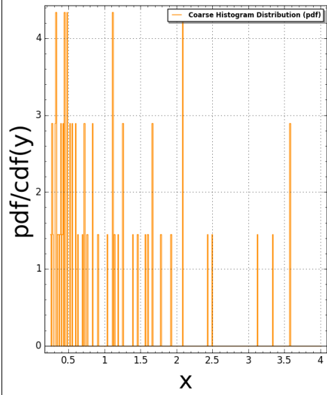
MiniTangram(N:=6) Slope Gaps: #bins=350, #tiling points = 353 Time Taken: 9.9961 sec (0.166602 mins)
