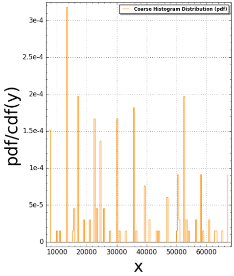
GRTriangle(N:=6) Pair Correlation (Squared): #bins=150, #tiling points = 53 Time Taken: 299.985 sec (4.99974 mins)
