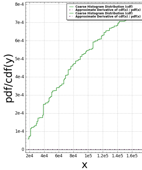
GRTriangle(N:=6) Pair Correlation (Squared): #bins=125, #tiling points = 53 Time Taken: 299.165 sec (4.98608 mins)
