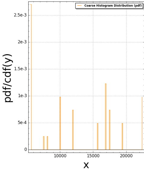
GRTriangle(N:=5) Pair Correlation (Squared): #bins=150, #tiling points = 23 Time Taken: 93.1673 sec (1.55279 mins)
