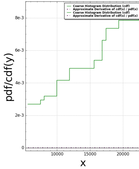
GRTriangle(N:=5) Pair Correlation (Squared): #bins=150, #tiling points = 23 Time Taken: 93.1673 sec (1.55279 mins)
