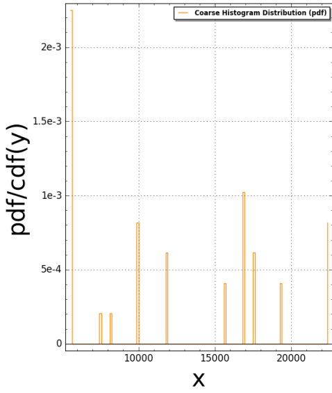
GRTriangle(N:=5) Pair Correlation (Squared): #bins=125, #tiling points = 23 Time Taken: 92.4615 sec (1.54103 mins)
