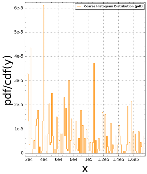
GRTriangle(N:=6) Pair Correlation (Squared): #bins=125, #tiling points = 53 Time Taken: 299.165 sec (4.98608 mins)
