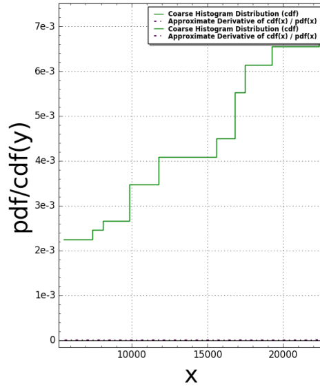
GRTriangle(N:=5) Pair Correlation (Squared): #bins=125, #tiling points = 23 Time Taken: 92.4615 sec (1.54103 mins)
