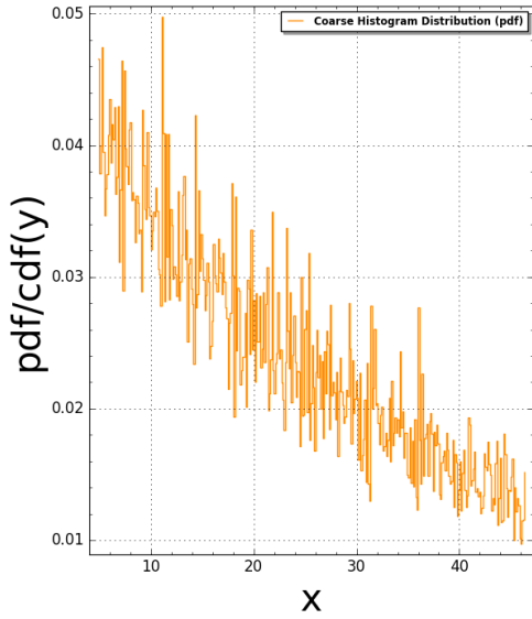
Fibonacci2D(N:=8) Pair Correlation (Squared): #bins=350, #tiling points = 1414 Time Taken: 32.4796 sec (0.541327 mins)
