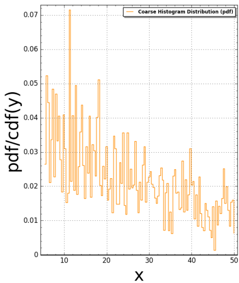
Fibonacci2D(N:=7) Pair Correlation (Squared): #bins=125, #tiling points = 557 Time Taken: 11.6139 sec (0.193565 mins)
