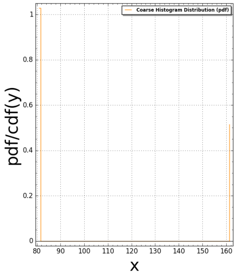
Fibonacci2D(N:=1) Pair Correlation (Squared): #bins=125, #tiling points = 4 Time Taken: 5.39303 sec (0.0898838 mins)
