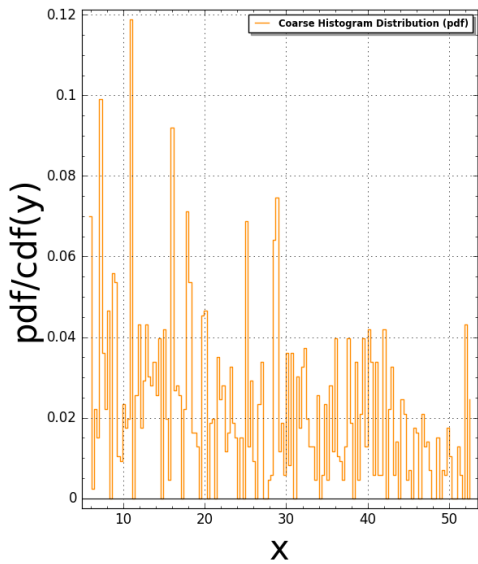
Fibonacci2D(N:=5) Pair Correlation (Squared): #bins=150, #tiling points = 92 Time Taken: 6.22196 sec (0.103699 mins)
