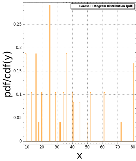
Fibonacci2D(N:=4) Pair Correlation (Squared): #bins=150, #tiling points = 40 Time Taken: 6.57362 sec (0.10956 mins)
