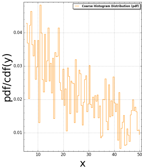
Fibonacci2D(N:=6) Pair Correlation (Squared): #bins=100, #tiling points = 224 Time Taken: 6.37855 sec (0.106309 mins)
