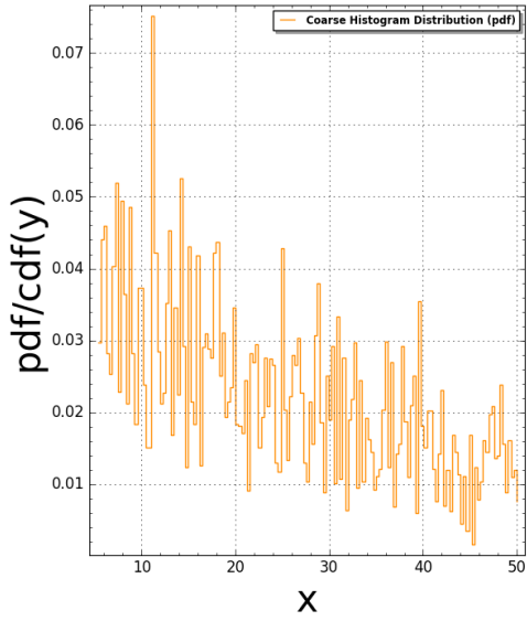
Fibonacci2D(N:=7) Pair Correlation (Squared): #bins=150, #tiling points = 557 Time Taken: 12.3395 sec (0.205659 mins)
