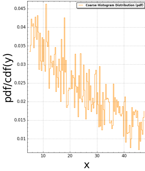
Fibonacci2D(N:=8) Pair Correlation (Squared): #bins=150, #tiling points = 1414 Time Taken: 28.7623 sec (0.479371 mins)
