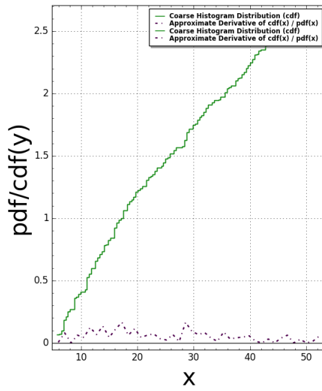
Fibonacci2D(N:=6) Pair Correlation (Squared): #bins=125, #tiling points = 224 Time Taken: 6.99138 sec (0.116523 mins)
