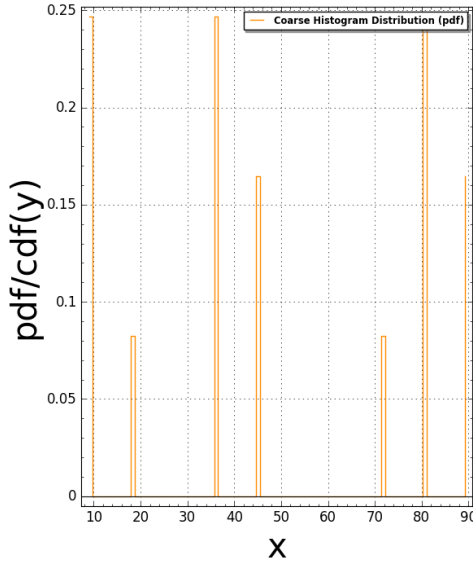
Fibonacci2D(N:=3) Pair Correlation (Squared): #bins=100, #tiling points = 17 Time Taken: 4.74282 sec (0.079047 mins)
