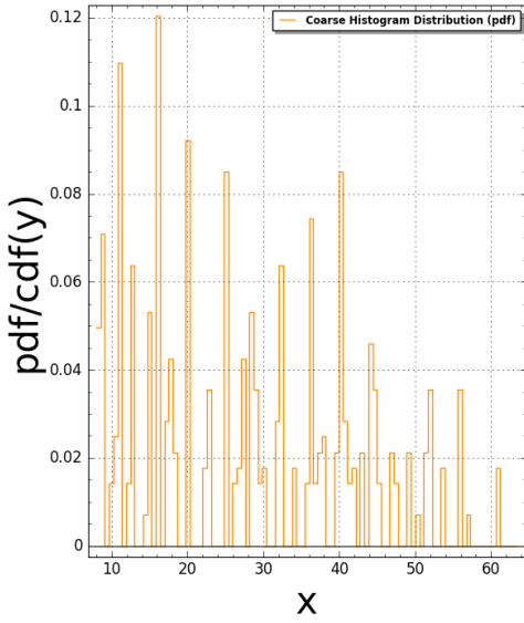
Fibonacci2D(N:=5) Pair Correlation (Squared): #bins=100, #tiling points = 92 Time Taken: 4.90578 sec (0.081763 mins)
