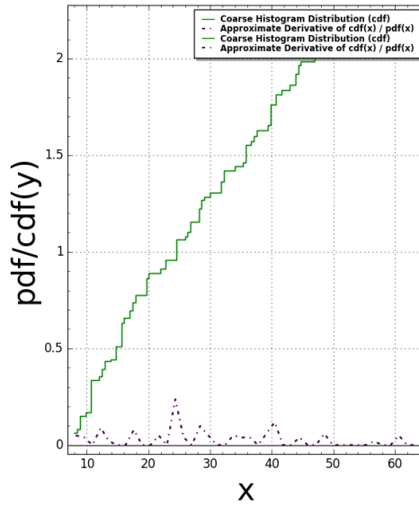
Fibonacci2D(N:=4) Pair Correlation (Squared): #bins=125, #tiling points = 40 Time Taken: 6.01885 sec (0.100314 mins)
