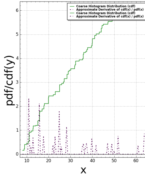
Fibonacci2D(N:=5) Pair Correlation (Squared): #bins=350, #tiling points = 92 Time Taken: 8.34506 sec (0.139084 mins)
