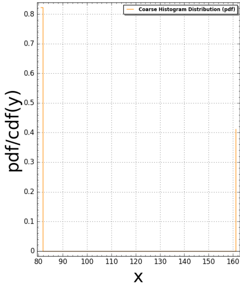
Fibonacci2D(N:=2) Pair Correlation (Squared): #bins=100, #tiling points = 9 Time Taken: 4.88369 sec (0.0813949 mins)
