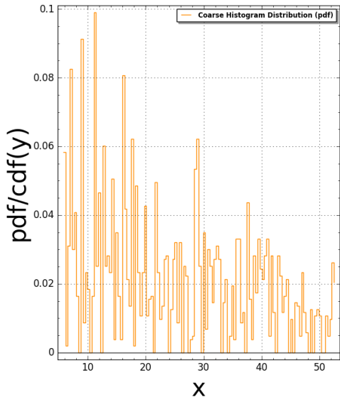
Fibonacci2D(N:=6) Pair Correlation (Squared): #bins=125, #tiling points = 224 Time Taken: 6.99138 sec (0.116523 mins)
