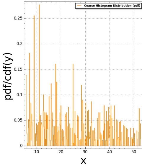
Fibonacci2D(N:=6) Pair Correlation (Squared): #bins=350, #tiling points = 224 Time Taken: 9.73979 sec (0.16233 mins)
