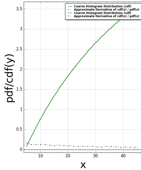
Fibonacci2D(N:=8) Pair Correlation (Squared): #bins=150, #tiling points = 1414 Time Taken: 28.7623 sec (0.479371 mins)
