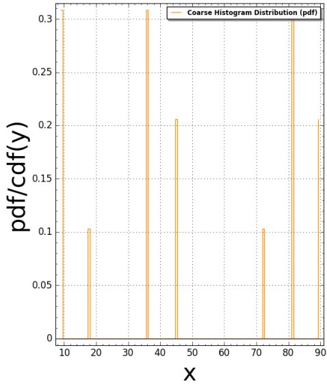
Fibonacci2D(N:=3) Pair Correlation (Squared): #bins=125, #tiling points = 17 Time Taken: 5.41339 sec (0.0902231 mins)
