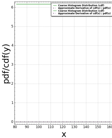
Fibonacci2D(N:=1) Pair Correlation (Squared): #bins=125, #tiling points = 4 Time Taken: 5.39303 sec (0.0898838 mins)
