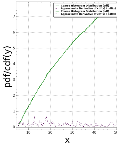
Fibonacci2D(N:=6) Pair Correlation (Squared): #bins=350, #tiling points = 224 Time Taken: 9.73979 sec (0.16233 mins)
