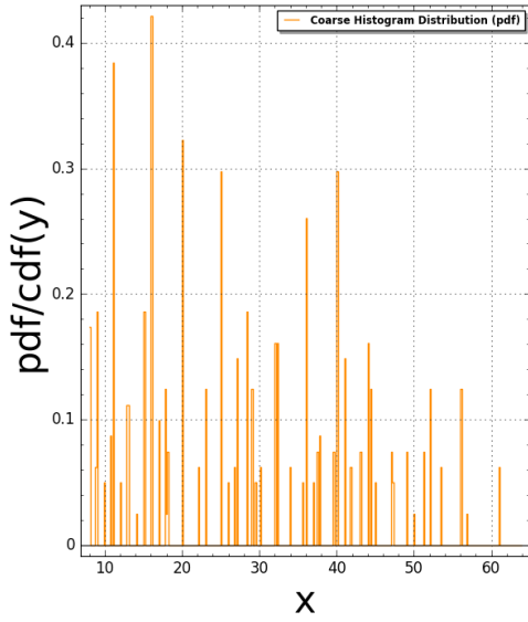
Fibonacci2D(N:=5) Pair Correlation (Squared): #bins=350, #tiling points = 92 Time Taken: 8.34506 sec (0.139084 mins)
