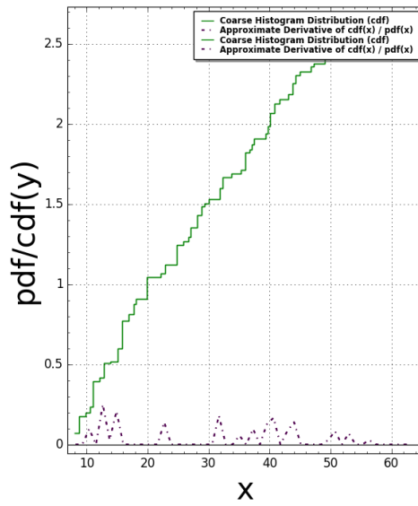
Fibonacci2D(N:=5) Pair Correlation (Squared): #bins=150, #tiling points = 92 Time Taken: 6.22196 sec (0.103699 mins)
