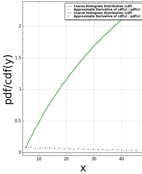
Fibonacci2D(N:=8) Pair Correlation (Squared): #bins=100, #tiling points = 1414 Time Taken: 26.384 sec (0.439733 mins)
