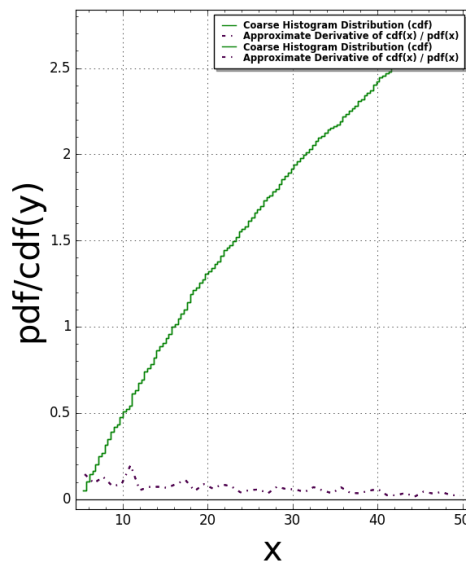
Fibonacci2D(N:=7) Pair Correlation (Squared): #bins=125, #tiling points = 557 Time Taken: 11.6139 sec (0.193565 mins)
