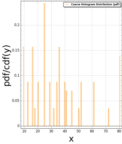
Fibonacci2D(N:=4) Pair Correlation (Squared): #bins=125, #tiling points = 40 Time Taken: 6.01885 sec (0.100314 mins)
