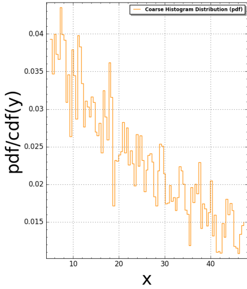
Fibonacci2D(N:=8) Pair Correlation (Squared): #bins=100, #tiling points = 1414 Time Taken: 26.384 sec (0.439733 mins)
