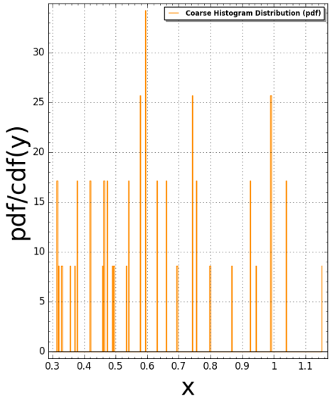
Equithirds(N:=6) Slope Gaps: #bins=350, #tiling points = 154 Time Taken: 29.8693 sec (0.497822 mins)
