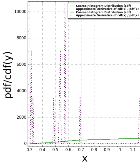
Equithirds(N:=6) Slope Gaps: #bins=350, #tiling points = 154 Time Taken: 29.8693 sec (0.497822 mins)
