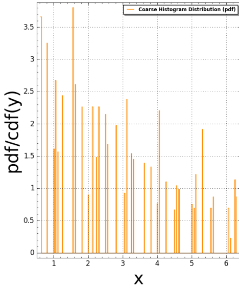
Domino(N:=5) Pair Correlation (Squared): #bins=350, #tiling points = 432 Time Taken: 12.6766 sec (0.211277 mins)
