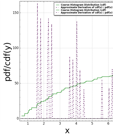
Domino(N:=5) Pair Correlation (Squared): #bins=350, #tiling points = 432 Time Taken: 12.6766 sec (0.211277 mins)
