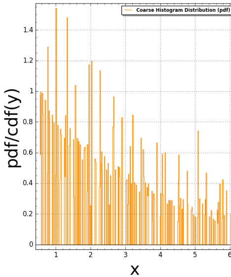
Domino(N:=6) Pair Correlation (Squared): #bins=350, #tiling points = 1682 Time Taken: 36.0692 sec (0.601154 mins)
