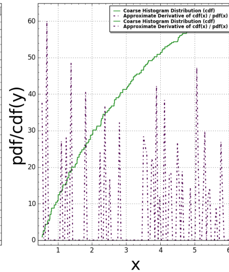
Domino(N:=6) Pair Correlation (Squared): #bins=350, #tiling points = 1682 Time Taken: 36.0692 sec (0.601154 mins)
