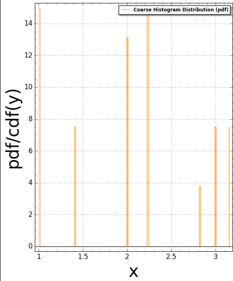
Domino(N:=3) Pair Correlation: #bins=150, #tiling points = 32 Time Taken: 5.29359 sec (0.0882265 mins)
