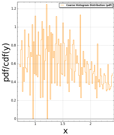
Domino(N=6) Pair Correlation: #bins=125, #tiling points = 1682 Time Taken: 29.2091 sec (0.486818 mins)
