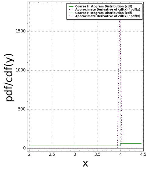
Domino(N:=1) Pair Correlation: #bins=150, #tiling points = 4 Time Taken: 5.34089 sec (0.0890149 mins)
