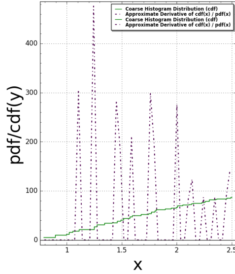
Domino(N:=4) Pair Correlation: #bins=150, #tiling points = 114 Time Taken: 5.63743 sec (0.0939571 mins)
