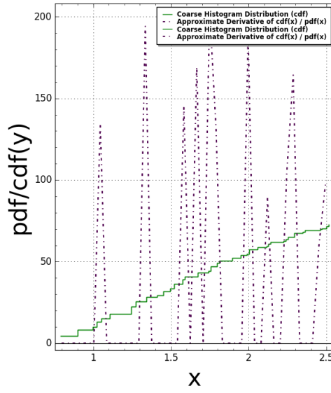
Domino(N=5) Pair Correlation: #bins=125, #tiling points = 432 Time Taken: 7.70325 sec (0.128387 mins)
