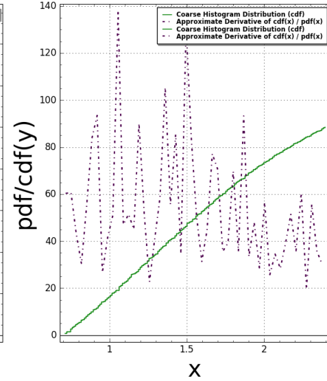
Domino(N:=6) Pair Correlation: #bins=150, #tiling points = 1682 Time Taken: 30.6801 sec (0.511336 mins)
