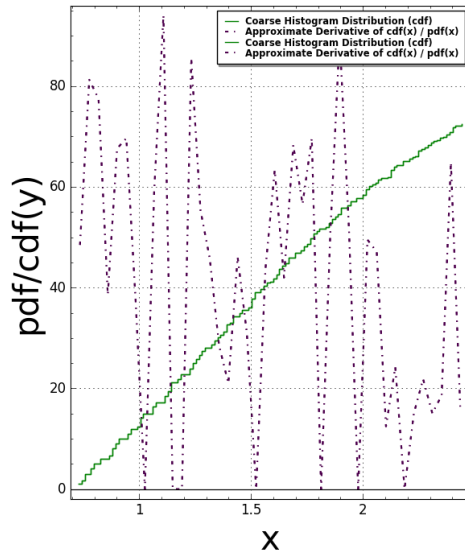
Domino(N=6) Pair Correlation: #bins=125, #tiling points = 1682 Time Taken: 29.2091 sec (0.486818 mins)
