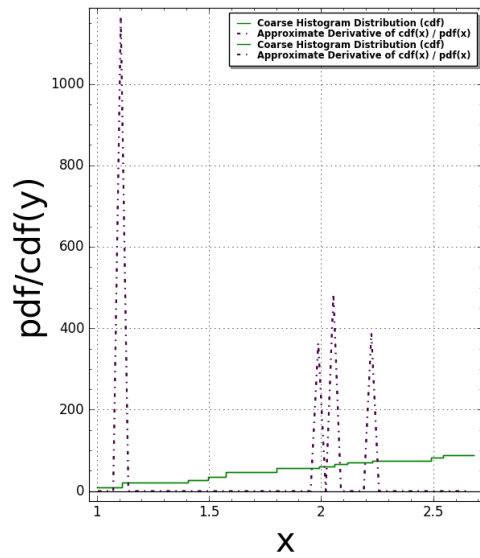
Domino(N:=3) Pair Correlation: #bins=150, #tiling points = 32 Time Taken: 5.29359 sec (0.0882265 mins)
