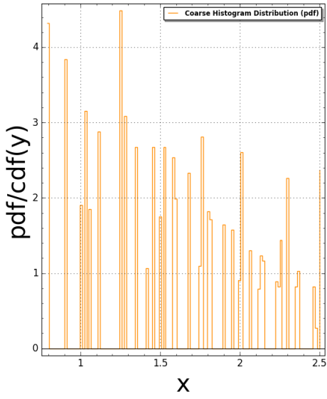
Domino(N=5) Pair Correlation: #bins=125, #tiling points = 432 Time Taken: 7.70325 sec (0.128387 mins)
