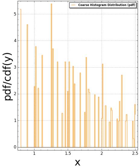
Domino(N:=4) Pair Correlation: #bins=150, #tiling points = 114 Time Taken: 5.63743 sec (0.0939571 mins)
