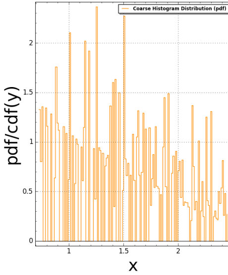
Domino(N:=6) Pair Correlation: #bins=150, #tiling points = 1682 Time Taken: 30.6801 sec (0.511336 mins)
