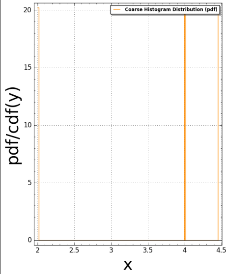
Domino(N:=1) Pair Correlation: #bins=150, #tiling points = 4 Time Taken: 5.34089 sec (0.0890149 mins)
