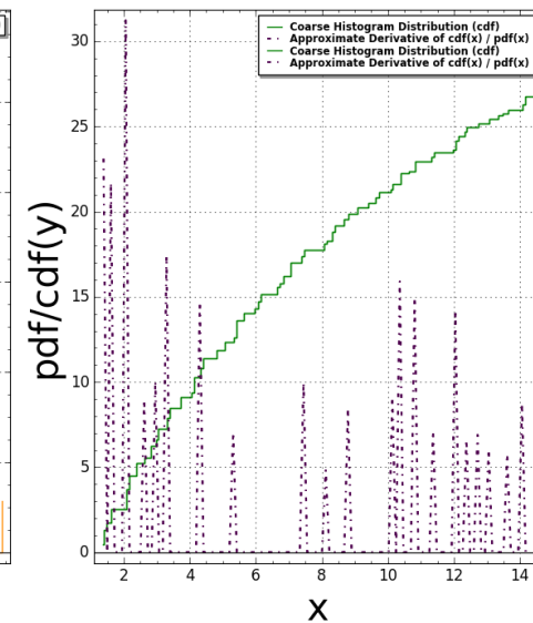
Chair3(N:=3) Pair Correlation (Squared): #bins=350, #tiling points = 286 Time Taken: 9.38691 sec (0.156448 mins)
