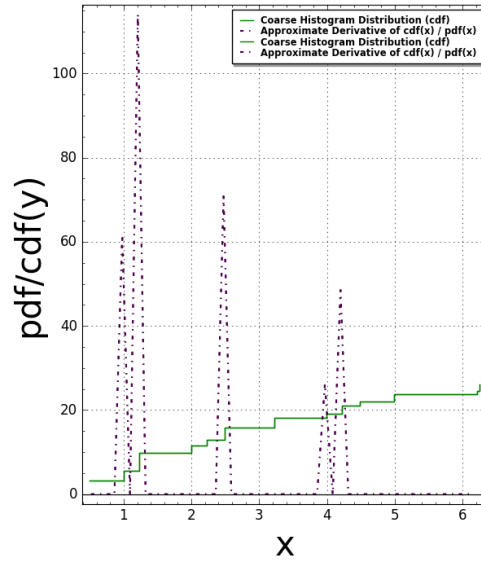
Chair3(N:=3) Pair Correlation (Squared): #bins=150, #tiling points = 286 Time Taken: 7.35489 sec (0.122582 mins)
