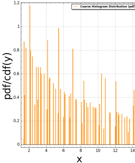
Chair3(N:=3) Pair Correlation (Squared): #bins=350, #tiling points = 286 Time Taken: 9.38691 sec (0.156448 mins)
