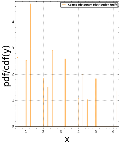
Chair3(N:=3) Pair Correlation (Squared): #bins=150, #tiling points = 286 Time Taken: 7.35489 sec (0.122582 mins)
