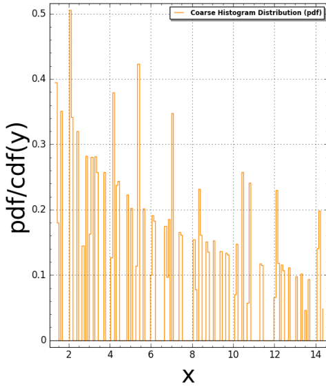
Chair3(N:=4) Pair Correlation (Squared): #bins=150, #tiling points = 2253 Time Taken: 42.5885 sec (0.709808 mins)
