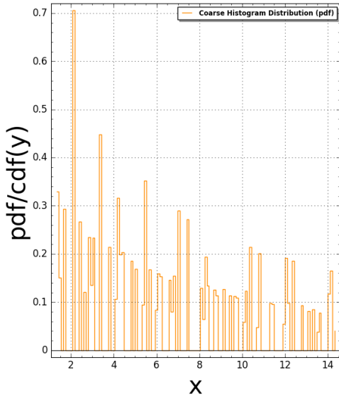
Chair3(N:=4) Pair Correlation (Squared): #bins=125, #tiling points = 2253 Time Taken: 39.6096 sec (0.660159 mins)
