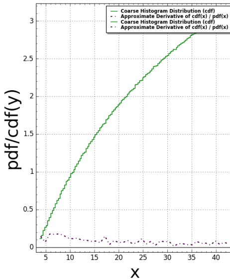
Chair3(N:=1) Pair Correlation (Squared): #bins=150, #tiling points = 6 Time Taken: 5.90795 sec (0.0984658 mins)
