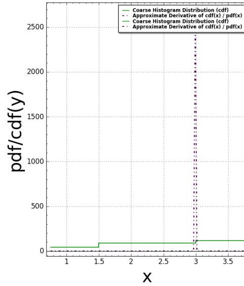
Chair3(N:=2) Pair Correlation (Squared): #bins=350, #tiling points = 38 Time Taken: 8.41102 sec (0.140184 mins)
