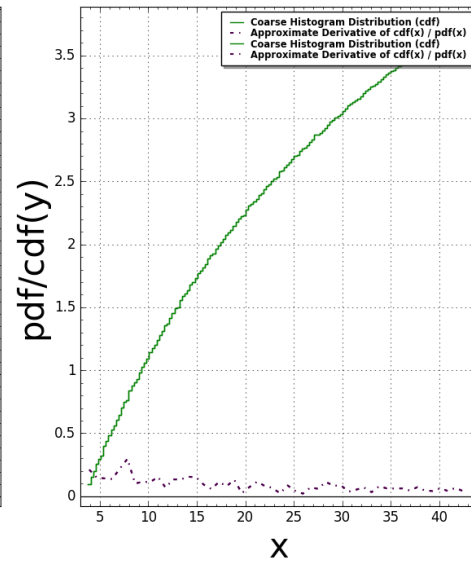
Chair3(N:=4) Pair Correlation (Squared): #bins=150, #tiling points = 2253 Time Taken: 42.5885 sec (0.709808 mins)
