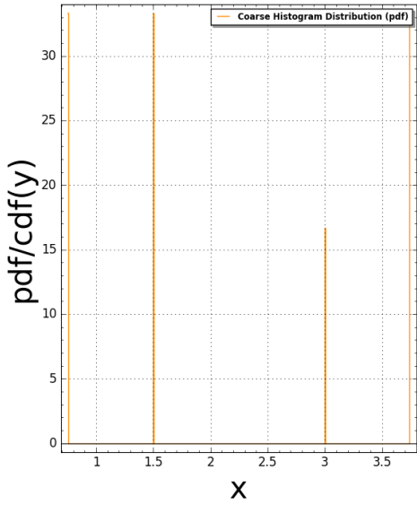
Chair3(N:=2) Pair Correlation (Squared): #bins=350, #tiling points = 38 Time Taken: 8.41102 sec (0.140184 mins)
