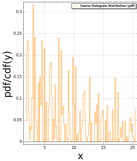
AmmannRhomb(N:=1) Pair Correlation (Squared): #bins=150, #tiling points = 4 Time Taken: 6.91532 sec (0.115255 mins)
