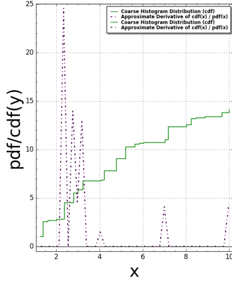
AmmannRhomb(N:=4) Pair Correlation (Squared): #bins=125, #tiling points = 199 Time Taken: 8.82558 sec (0.147093 mins)
