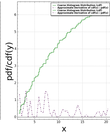
AmmannRhomb(N:=1) Pair Correlation (Squared): #bins=150, #tiling points = 4 Time Taken: 6.91532 sec (0.115255 mins)
