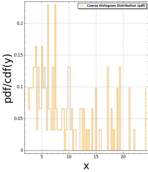
AmmannEightStar(N:=1) Slope Gaps: #bins=125, #tiling points = 17 Time Taken: 7.37217 sec (0.12287 mins)
