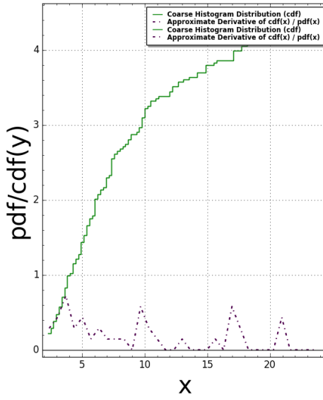
AmmannEightStar(N:=1) Slope Gaps: #bins=125, #tiling points = 17 Time Taken: 7.37217 sec (0.12287 mins)
