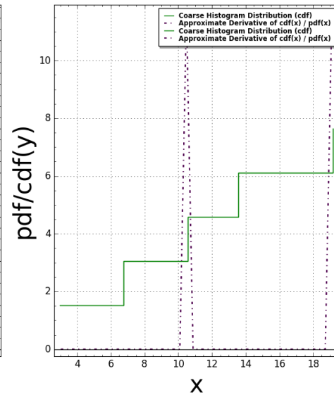
AmmannEightStar(N:=2) Slope Gaps: #bins=125, #tiling points = 57 Time Taken: 7.76357 sec (0.129393 mins)
