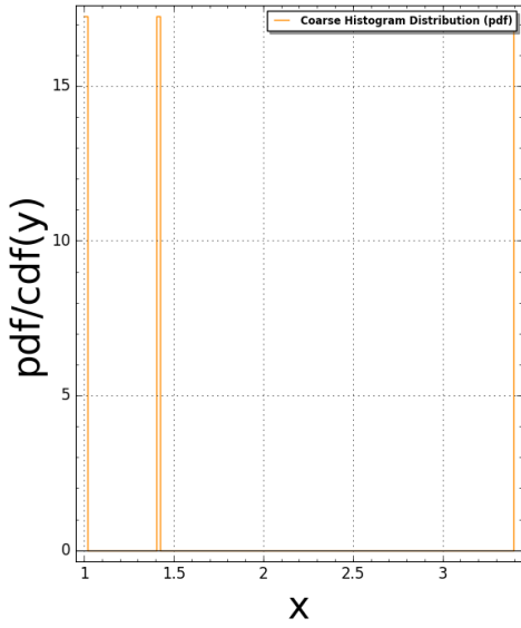
AmmannEightStar(N:=2) Slope Gaps: #bins=125, #tiling points = 57 Time Taken: 7.76357 sec (0.129393 mins)
