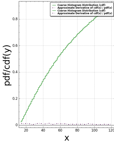
AmmannEightStar(N:=1) Pair Correlation (Squared): #bins=125, #tiling points = 17 Time Taken: 8.55748 sec (0.142625 mins)
