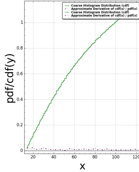
AmmannEightStar(N:=1) Pair Correlation (Squared): #bins=150, #tiling points = 17 Time Taken: 9.21398 sec (0.153566 mins)
