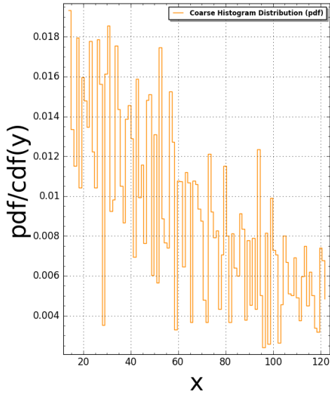
AmmannEightStar(N:=1) Pair Correlation (Squared): #bins=125, #tiling points = 17 Time Taken: 8.55748 sec (0.142625 mins)
