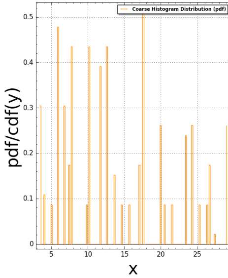
AmmannEightStar(N:=3) Pair Correlation (Squared): #bins=150, #tiling points = 289 Time Taken: 12.2894 sec (0.204823 mins)
