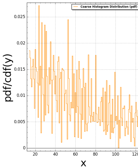
AmmannEightStar(N:=4) Pair Correlation (Squared): #bins=150, #tiling points = 1561 Time Taken: 69.2443 sec (1.15407 mins)
