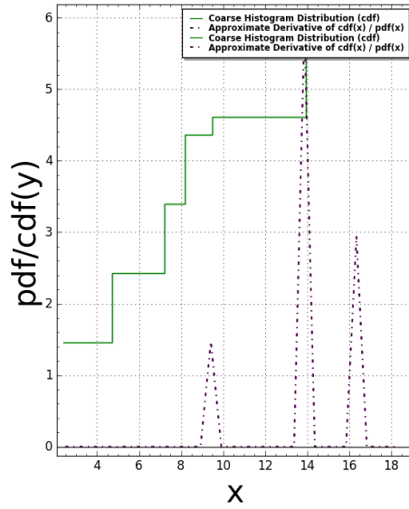
AmmannEightStar(N:=2) Pair Correlation (Squared): #bins=100, #tiling points = 57 Time Taken: 6.76817 sec (0.112803 mins)
