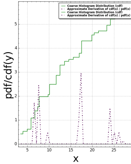
AmmannEightStar(N:=3) Pair Correlation (Squared): #bins=150, #tiling points = 289 Time Taken: 12.2894 sec (0.204823 mins)
