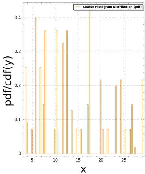
AmmannEightStar(N:=2) Pair Correlation (Squared): #bins=125, #tiling points = 57 Time Taken: 7.60107 sec (0.126684 mins)
