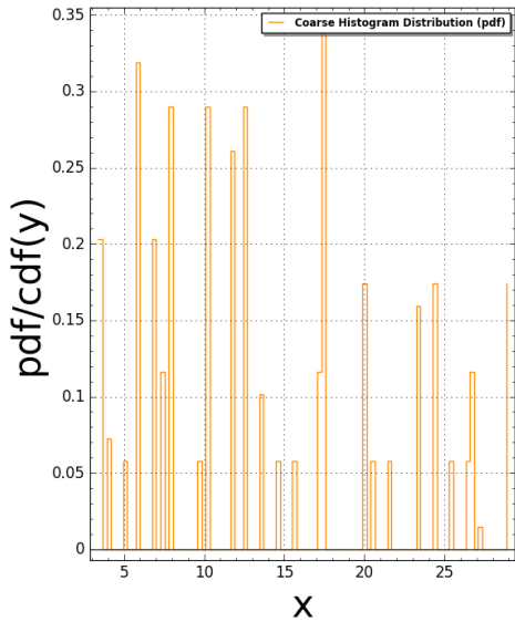
AmmannEightStar(N:=3) Pair Correlation (Squared): #bins=100, #tiling points = 289 Time Taken: 10.7507 sec (0.179178 mins)
