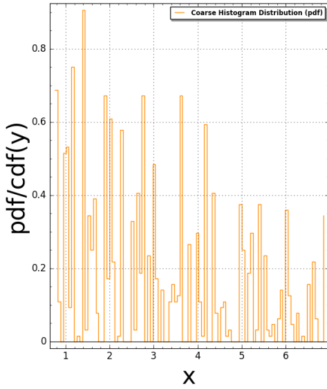
AmmannA3(N:=1) Pair Correlation (Squared): #bins=125, #tiling points = 6 Time Taken: 5.43046 sec (0.0905077 mins)
