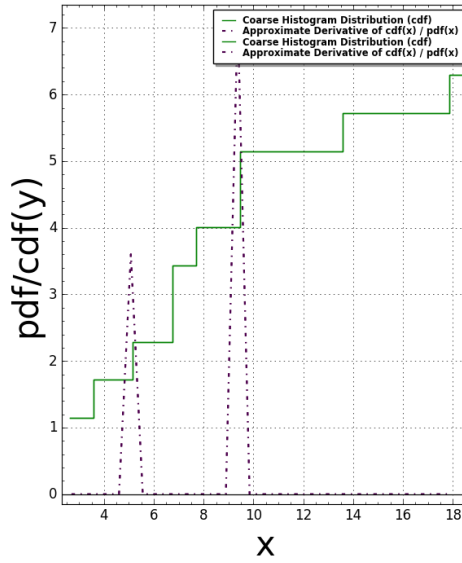
AmmannA3(N:=2) Pair Correlation (Squared): #bins=100, #tiling points = 10 Time Taken: 5.70211 sec (0.0950352 mins)
