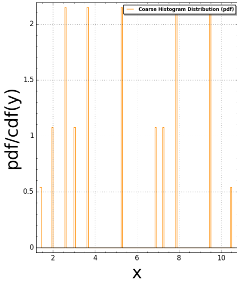
AmmannA3(N:=3) Pair Correlation (Squared): #bins=150, #tiling points = 24 Time Taken: 7.34478 sec (0.122413 mins)
