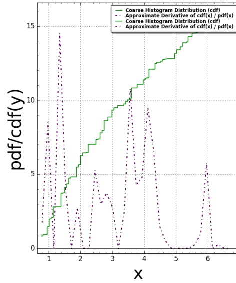
AmmannA3(N:=1) Pair Correlation (Squared): #bins=125, #tiling points = 6 Time Taken: 5.43046 sec (0.0905077 mins)
