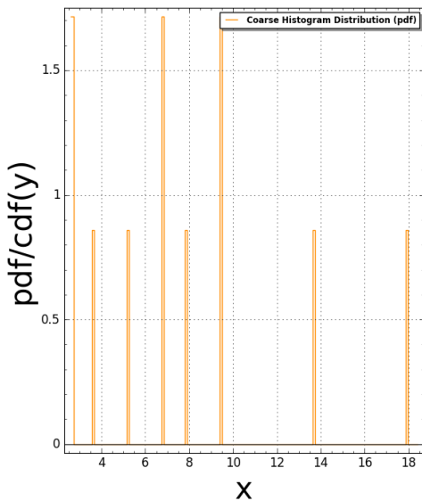
AmmannA3(N:=1) Pair Correlation (Squared): #bins=150, #tiling points = 6 Time Taken: 6.2519 sec (0.104198 mins)
