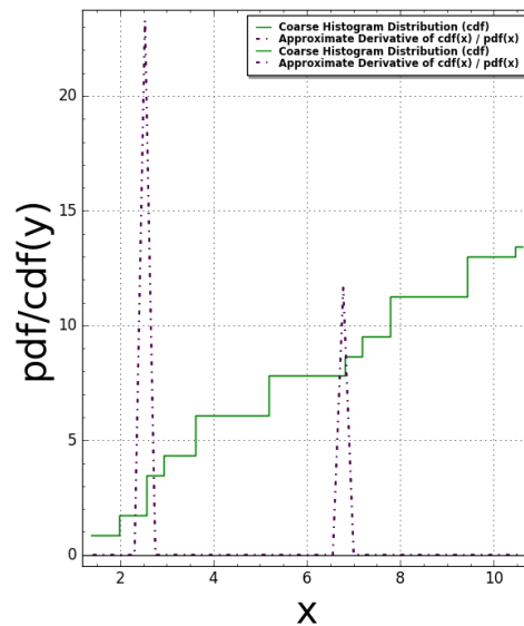
AmmannA3(N:=2) Pair Correlation (Squared): #bins=125, #tiling points = 10 Time Taken: 6.40801 sec (0.1068 mins)
