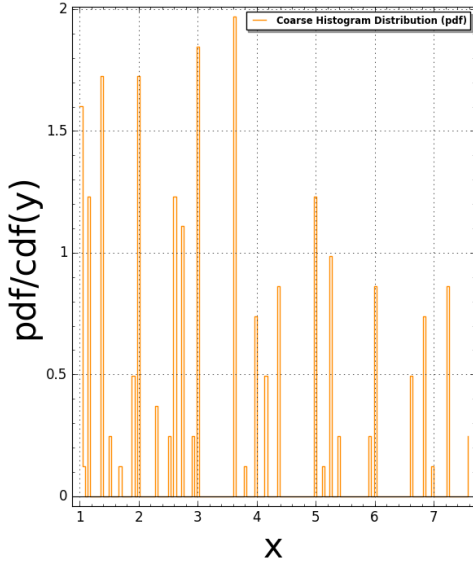
AmmannA3(N:=4) Pair Correlation (Squared): #bins=150, #tiling points = 57 Time Taken: 7.84544 sec (0.130757 mins)
