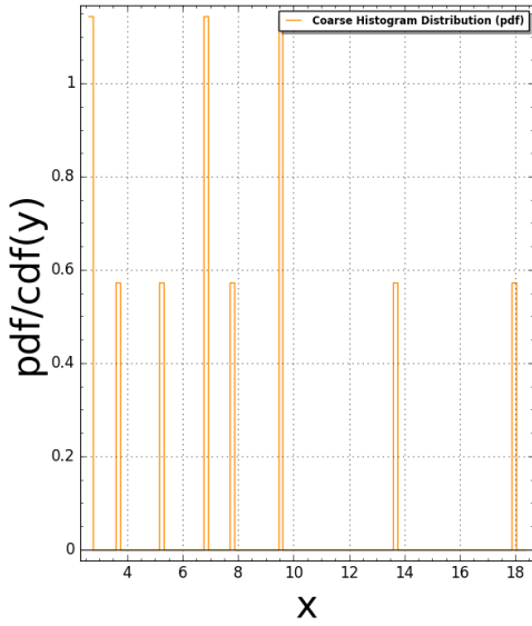
AmmannA3(N:=2) Pair Correlation (Squared): #bins=100, #tiling points = 10 Time Taken: 5.70211 sec (0.0950352 mins)
