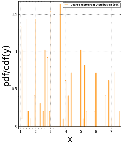
AmmannA3(N:=4) Pair Correlation (Squared): #bins=125, #tiling points = 57 Time Taken: 6.97242 sec (0.116207 mins)
