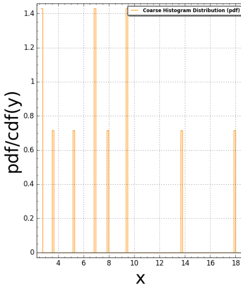
AmmannA3(N:=2) Pair Correlation (Squared): #bins=125, #tiling points = 10 Time Taken: 6.40801 sec (0.1068 mins)
