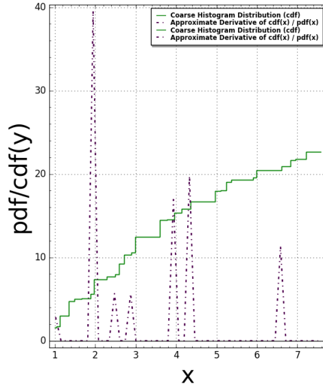
AmmannA3(N:=4) Pair Correlation (Squared): #bins=150, #tiling points = 57 Time Taken: 7.84544 sec (0.130757 mins)
