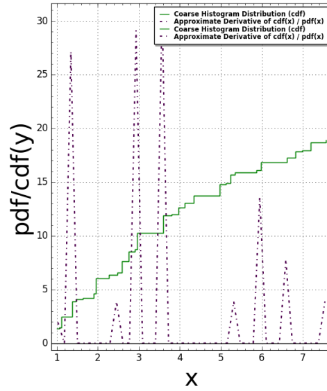
AmmannA3(N:=4) Pair Correlation (Squared): #bins=125, #tiling points = 57 Time Taken: 6.97242 sec (0.116207 mins)
