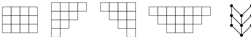
Figure 1: Examples of the families of posets to which Theorem 1 applies.
