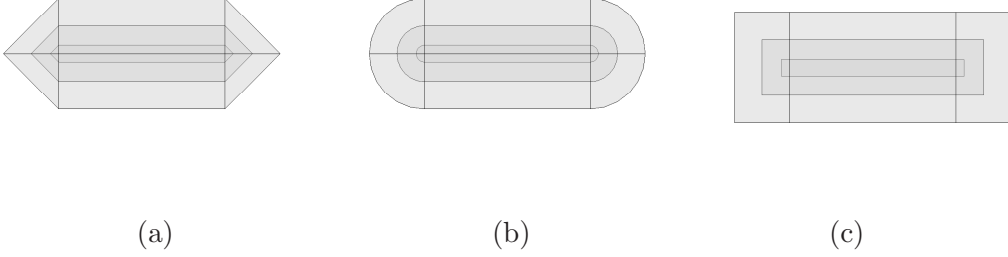
Figure 1: Two dimensional ABC geometry \mathbf{C} depicted in both the virtual space (between innermost and outermost boundaries) and the physical space (between intermediate and outermost boundaries). From left to right: l^1 , l^2 and l^\infty cloaks, respectively.
