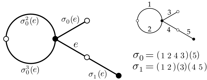
Figure 15: Left: The effect of \sigma_0 on edges. Right: the permutations \sigma_0 and \sigma_1 .
