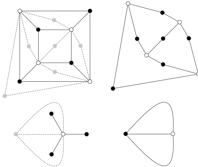
Figure 13: Taking the dual of the cube graph (top) and 3-star (bottom). Note the multiple edges introduced in the latter case.
