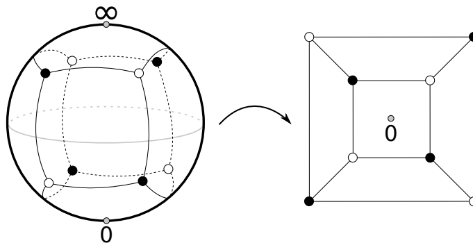
Figure 7: Mapping the cube graph from the sphere to the plane. The top face on the left, which contains \infty , becomes the outside face on the right.
