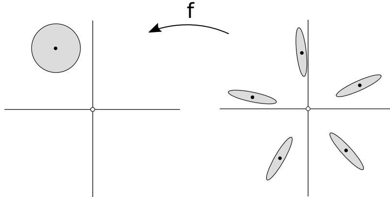
Figure 2: The n th power map f : \mathbb{C} \setminus \{0\} \rightarrow \mathbb{C} \setminus \{0\} sending z \mapsto z^n , seen here with n = 5 , is a covering map.
