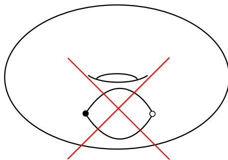
Figure 6: This is not a valid dessin d'enfant. Removing the graph produces two connected components; while one is homeomorphic to a disk, the other has a handle in it.
