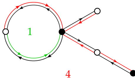
Figure 10: Counting the degrees of faces. Each edge here is doubled to account for the two faces it borders (though they may be the same face) and oriented in the direction associated with a counterclockwise walk around the boundary of that face. We then count only the edges which go from a white to a black vertex. Note that the walk around the outer face appears to be clockwise in this representation, but goes counterclockwise when it is viewed on the sphere.
