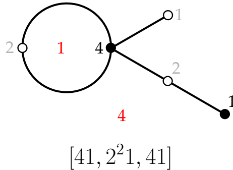
Figure 12: A plane dessin, its vertices and faces (red) labeled with their degrees. From this information, we obtain its passport.
