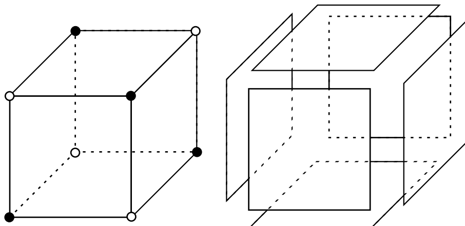
Figure 5: A cube graph embedded on a sphere (that is, a cube), and its faces.
