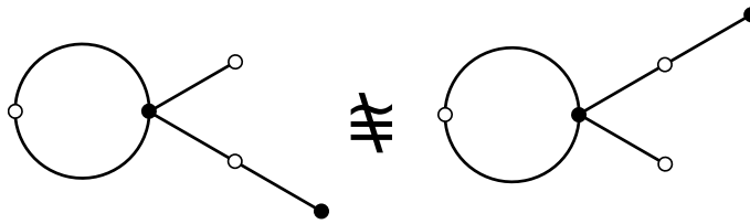
Figure 9: These dessins are not isomorphic.
