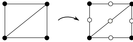
Figure 11: Converting an ordinary graph into a clean dessin.
