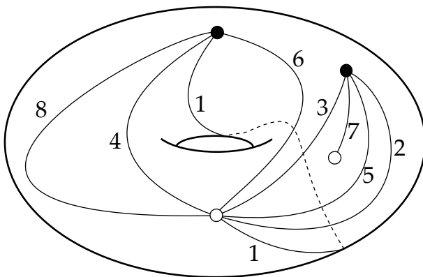
Figure 18: The result of Figure 17 on the more familiar representation of a torus. Observe that the associated permutations are \sigma_0 = (1\ 6\ 8\ 4)(2\ 3\ 7\ 5) and \sigma_1 = (1\ 2\ 5\ 3\ 6\ 4\ 8)(7) , the ones we started with.
