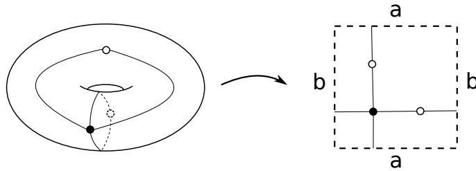
Figure 8: Depicting a dessin embedded on a torus. Note that it has only one face.
