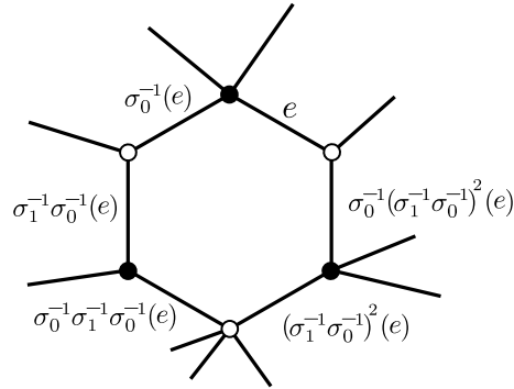
Figure 16: The permutation \sigma_\infty := \sigma_1^{-1}\sigma_0^{-1} .
