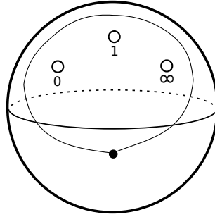
Figure 19: The product [\gamma_0][\gamma_1][\gamma_\infty] . Imagine pulling it around the back of the sphere.
