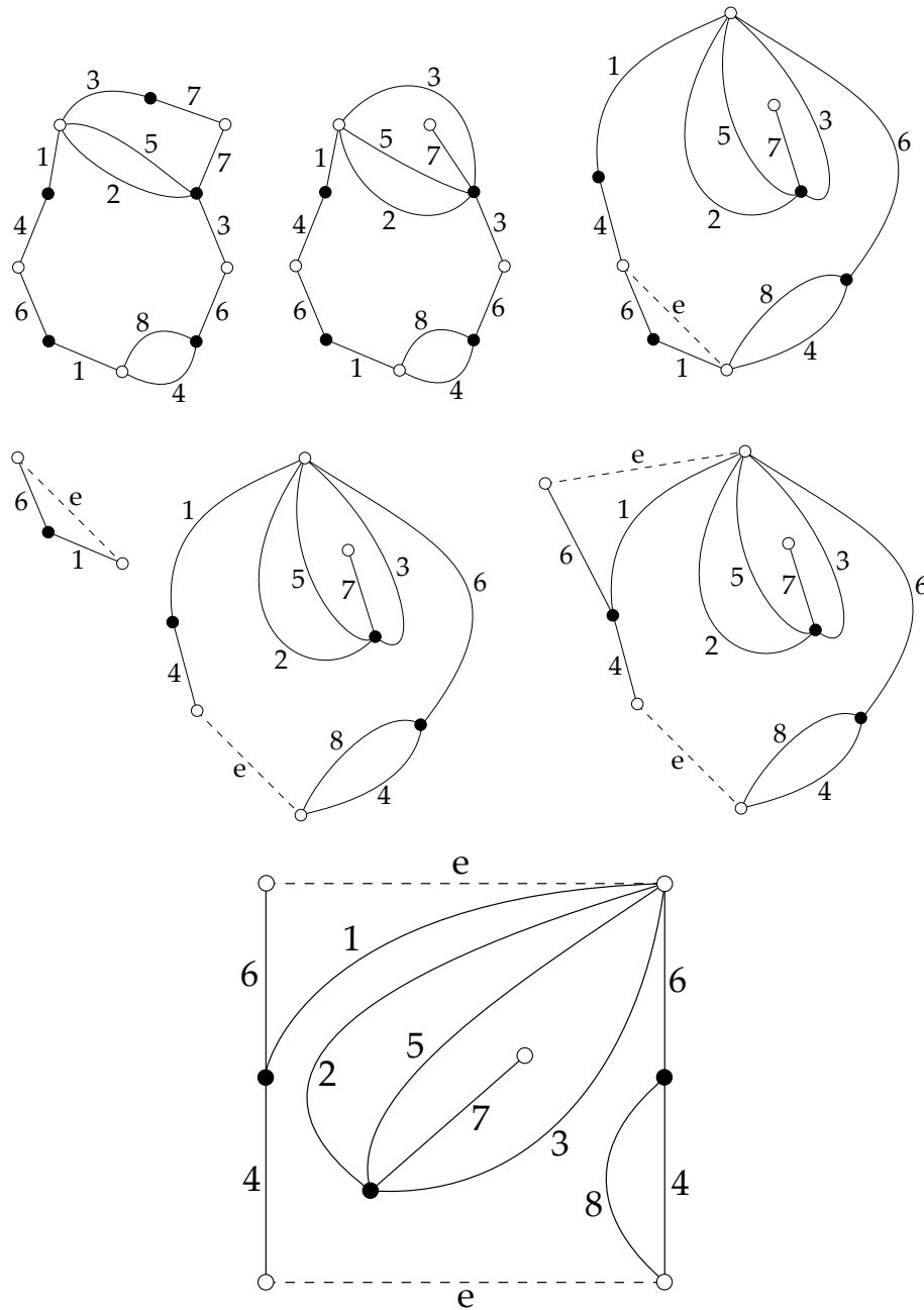
Figure 17: Transforming the above collection of faces into a representation of a dessin on a torus: collapsing the adjacent 7s inward, collapsing the adjacent 3s inward, cutting along the line e , reattaching at edge 1, and finally formatting the whole thing in a more sensible-looking representation.
