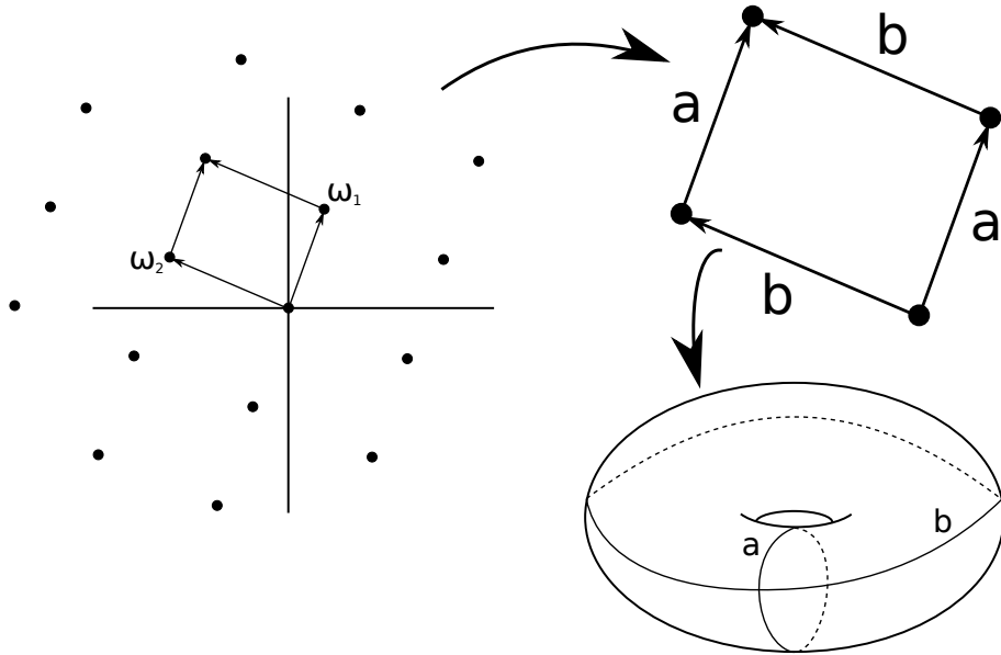
Figure 4: Constructing a torus as a quotient of the complex plane by the lattice generated by \omega_1 and \omega_2 .
