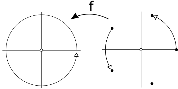
Figure 3: Lifting the circular loop around the origin along the covering map f sending z \mapsto z^5 , with a couple of different starting points.
