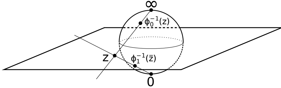
Figure 1: The Riemann sphere, with its two charts \varphi_0 and \varphi_1 .
