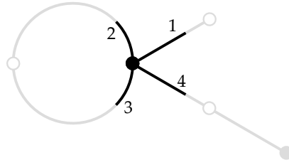
Figure 14: The ordering of edges around a vertex.
